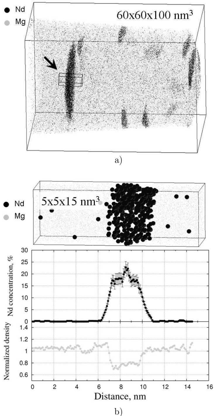
Figure 2.3.2: Atom probe analysis in the Mg-Nd alloy aged at 250^\circ\text{C} for 30 min. a) atom map; b) composition and atom number density profile across the interface indicated in (a) by the arrow.
