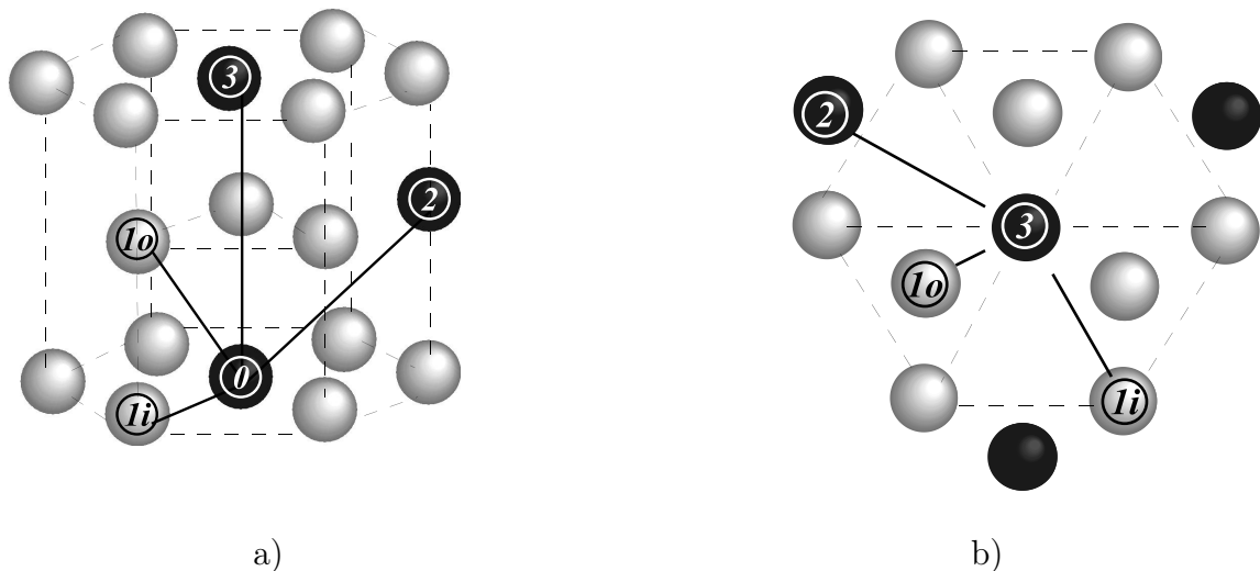
Figure 5.1.1: Perspective view a) and top view b) of the D0 19 ordered structure. The i^{\text{th}} neighbors of the 0-atom are denoted by the encircled number i . Black atoms are of type A and the gray ones are of type B.
