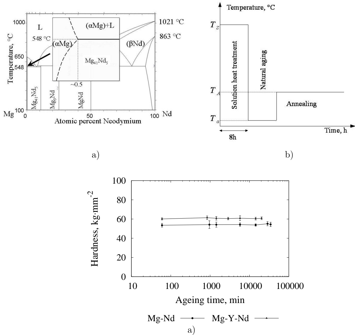
Figure 2.1.1: a) The binary Mg-Nd phase diagram [Oka07]. The inset shows schematically the Mg-rich side of the phase diagram. The solubility limit and eutectic temperature are taken from References [Rok62] and [Oka07]. b) Typical heat treatment sequence. T_S is the temperature of a homogenization; T_A is the temperature of a heat aging; T_a is the room temperature. c) The evolution of hardness in the homogenized Mg-Nd and Mg-Y-Nd alloys at room temperature (natural aging).
