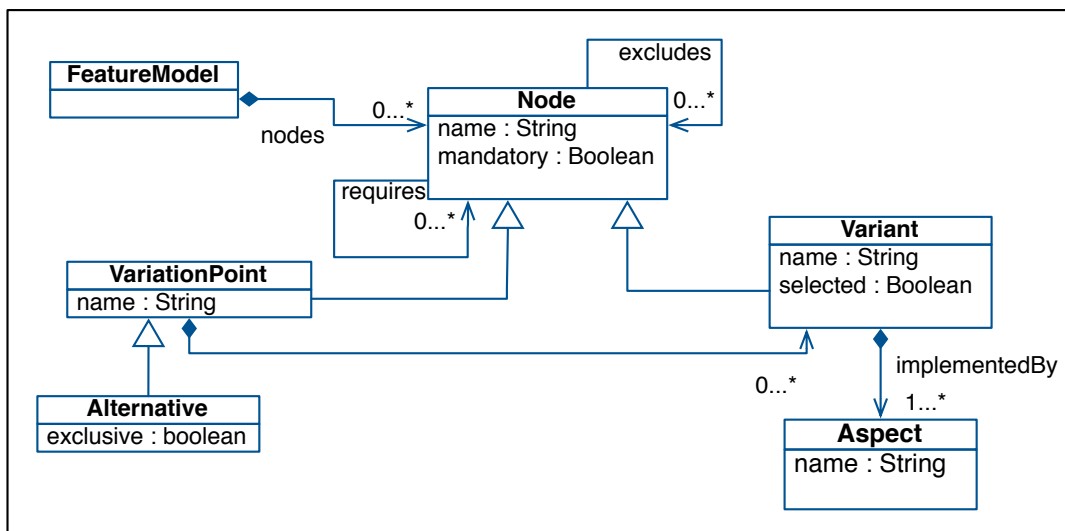
Figure 5.1: Feature metamodel.
