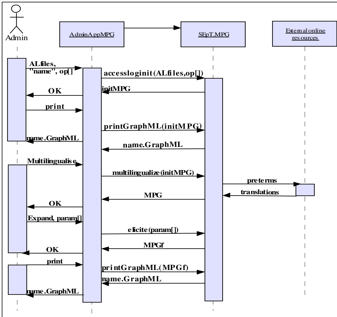
Fig. 66: Construction scenario
