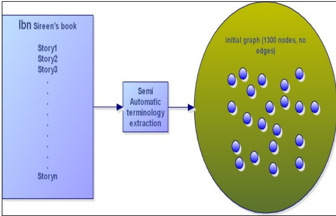
Fig. 74: MPG-Tafseer initialization
