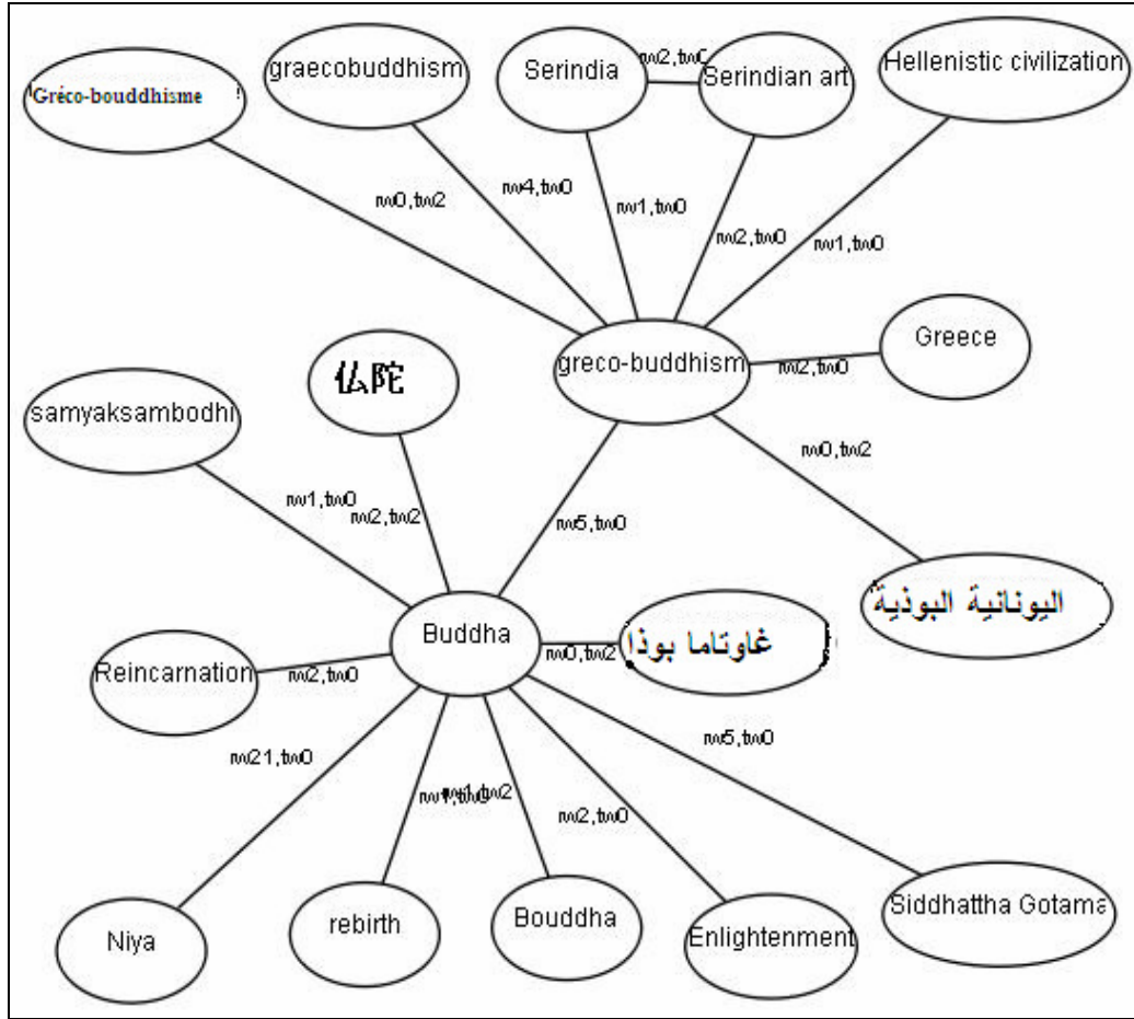
Fig. 68: Sample graph
