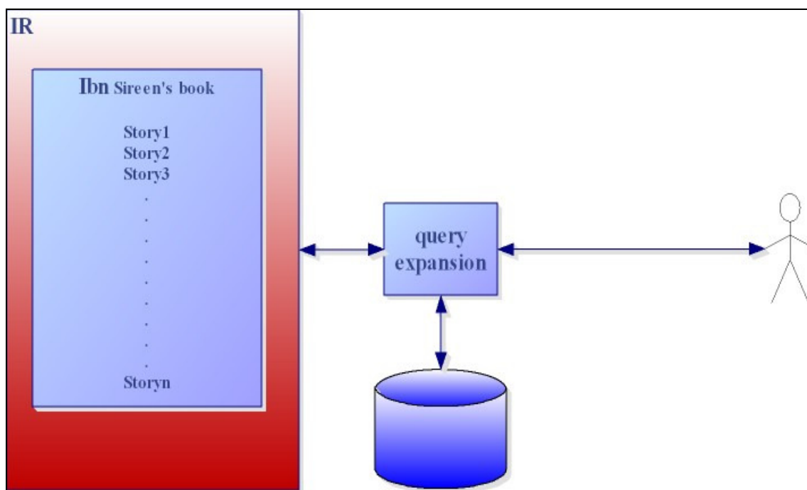
Fig. 73: Query expansion
