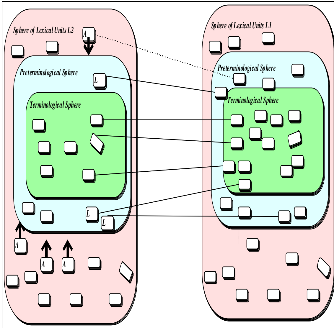
Fig. 25: Preterminological gap
