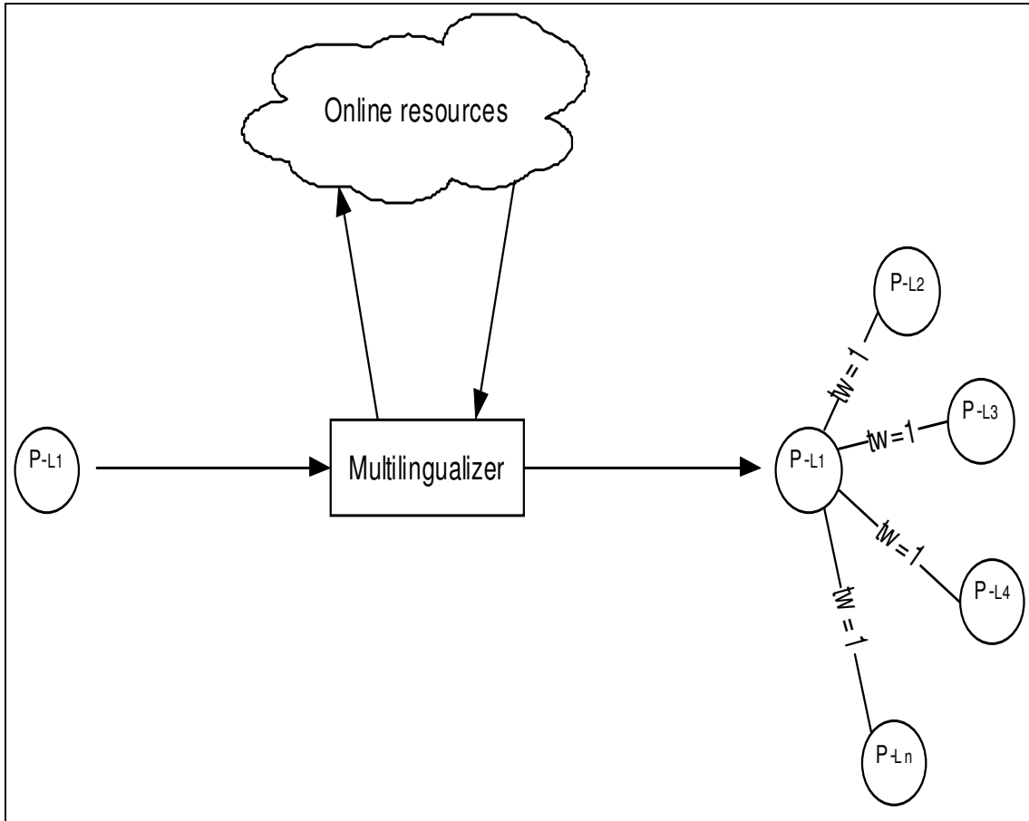
Fig. 42: Preterminology multilingualization
