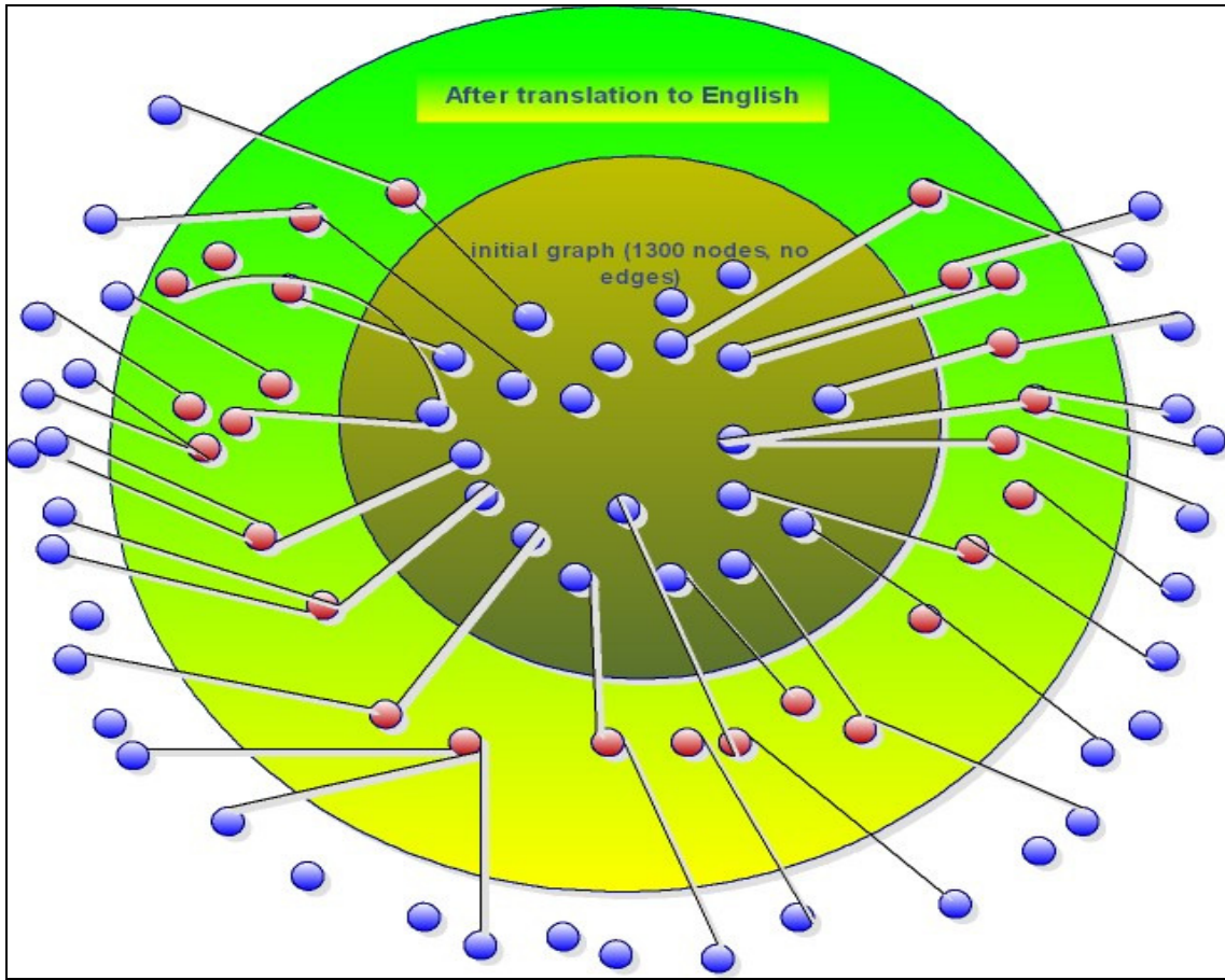
Fig. 75: MPG-Tafseer, Multilingualization
