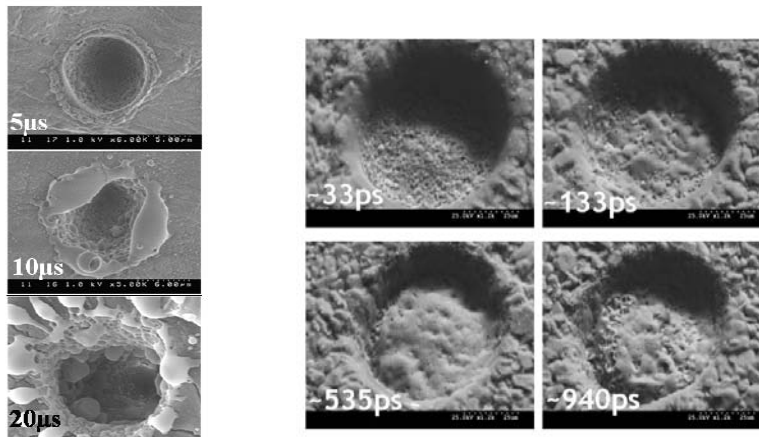
Figure 3.16 Burst mode ablation of tooth with ultrashort pulsetrain-bursts with 5,10 and 20 μs (From [61]) and alumina ceramic. (produced by Laser plasma lab, From [65])
