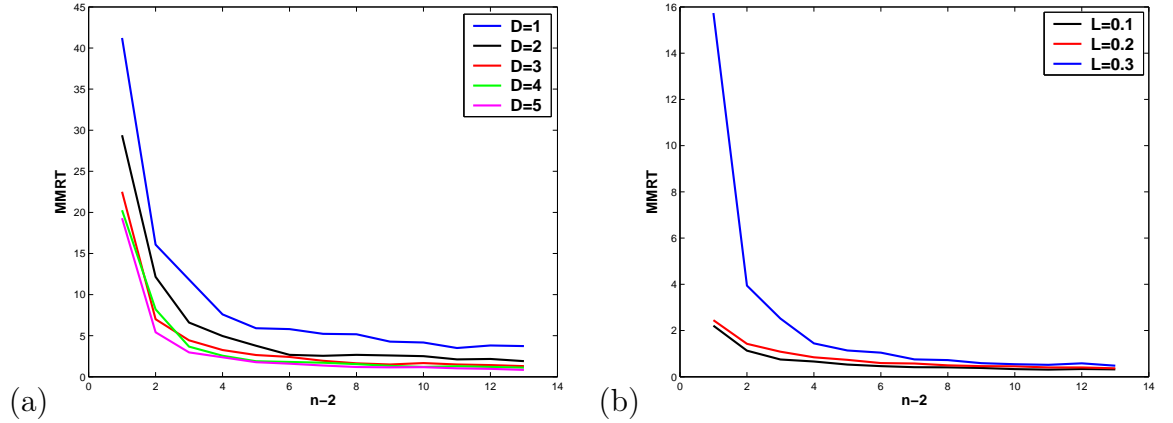
Figure 3.6: Brownian simulation of the MMRT as a function of the number of beads n - 2 . (a) For several values of D with L = 0.3 , (b) for several values of L with D = 10 .
