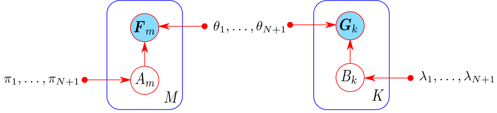
Figure 4.1: Graphical representation of a general conjugate mixture model. Circles denote random variables, plates (rectangles) around them represent multiple similar nodes, their number being given in the plates.
