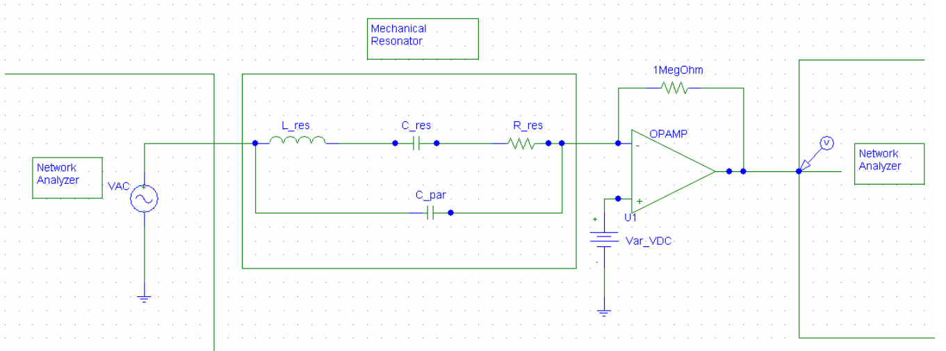
Fig. 3.15 The setup to measure the Q-factor
