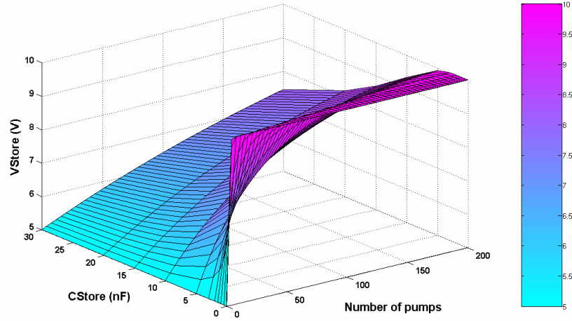
Fig. 2.5 Evolution of V_{Store} with C_{store} and number of pump cycles ( C_{Res} = 1 \mu F , C_{min} = 100 \text{ pF} )
