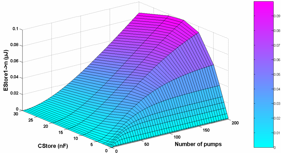
Fig. 2.6 Evolution of \Delta E_{1 \rightarrow n} with C_{store} and number of pump cycles ( C_{Res} = 1 \mu F , C_{min} = 100 \text{ pF} )
