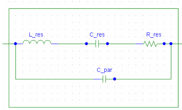
Fig. 3.14 Electrical representation of the resonator
