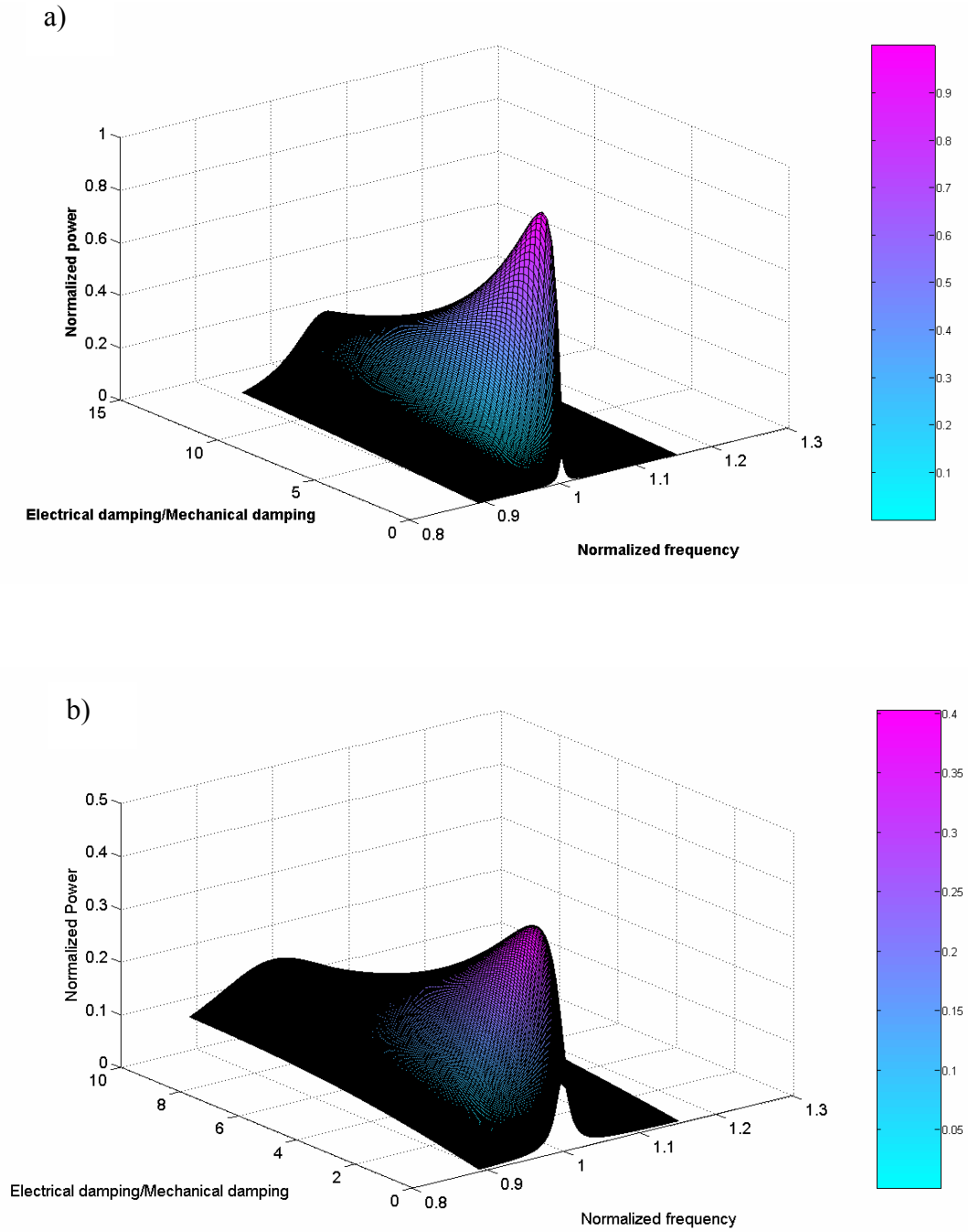
Fig. 1.8 a) Normalized power for system shown in Fig. 1.7 and using equation (1.3) b) Normalized power for system shown in Fig. 1.7 and using equation (1.3) with 1/3^{rd} the Q -factor, normalization is done with the maximum power generated in Fig. 1.8 (a)
