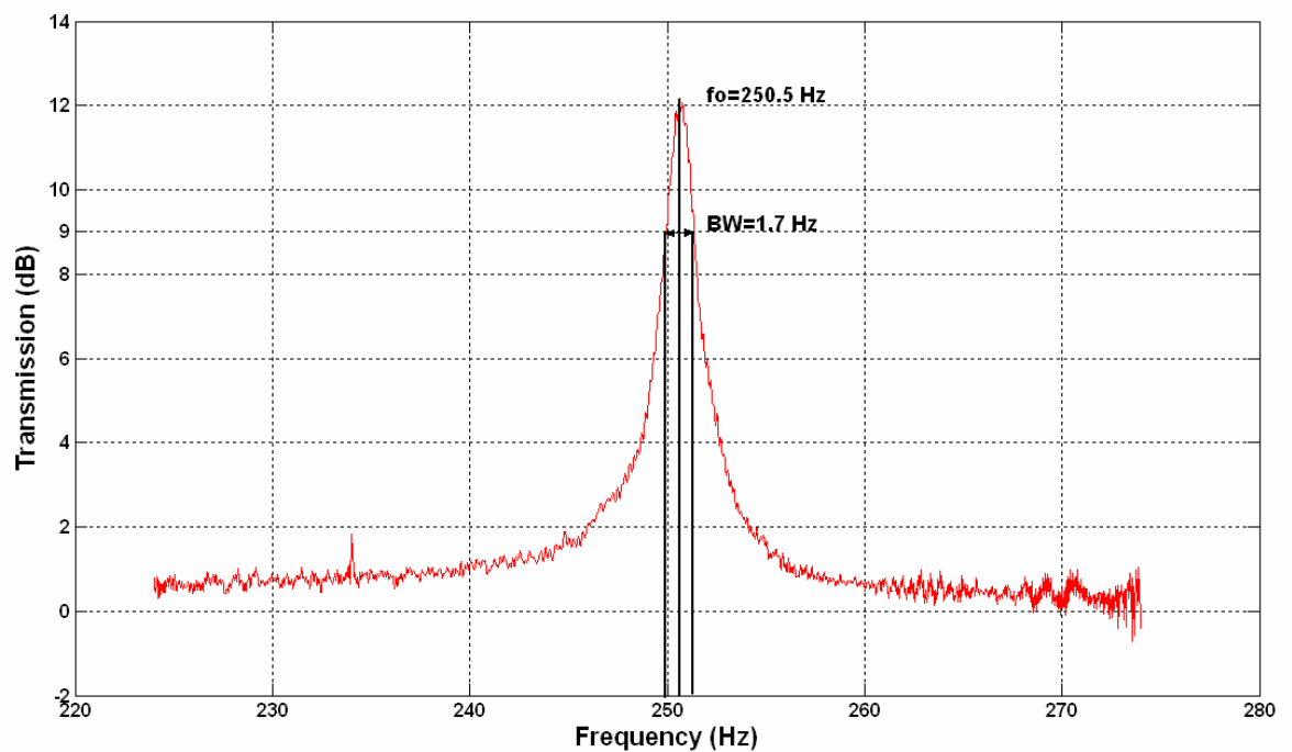
Fig. 3.17 Response of the resonator
