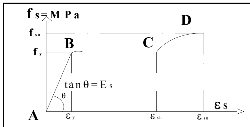
Figure 31 Stress-Strain diagram of the steel. [52]
