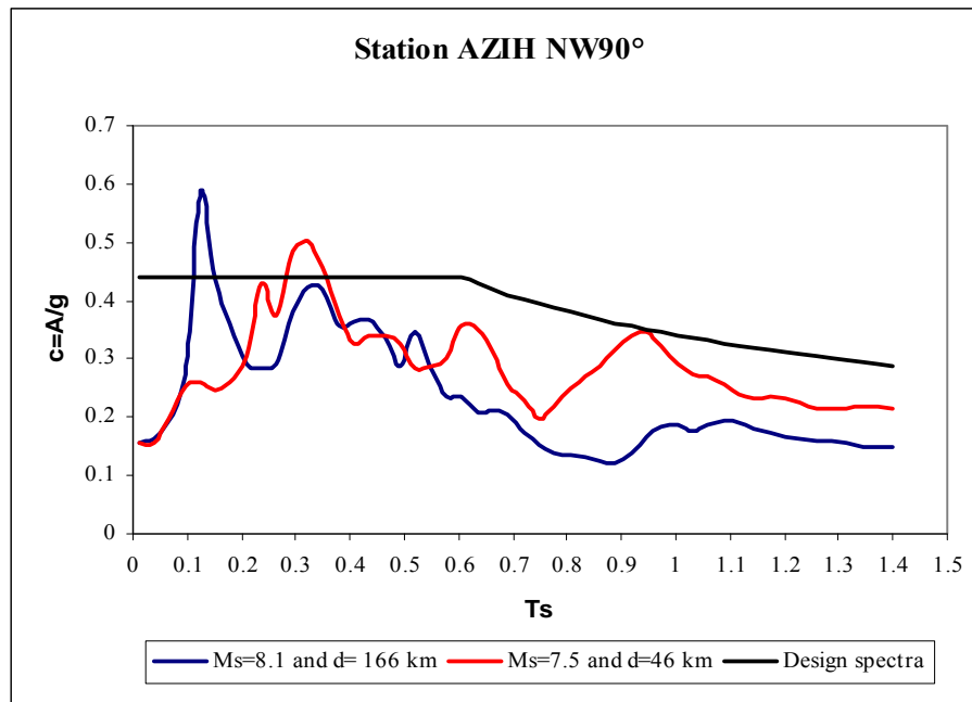
Figure 47 Site effects in the station AZIH with different magnitude and distances from station to the epicenter.
