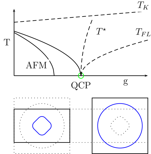
Figure 1.9: Scheme of an “unconventional” scenario for quantum criticality or Kondo breakdown. In this scenario again the Kondo energy is unchanged at the transition, but the Kondo lattice is and a characteristic energy scale of this domain vanishes. A magnetic order may or may not appears at this QCP depending on the model. The Fermi surface volume changes from small to large at the transition.
