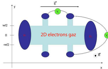
Figure 3.1: Hall bar
