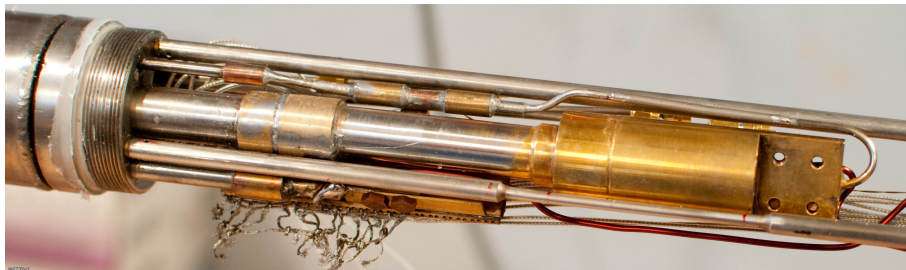
Figure 10.4: 1K Pot
