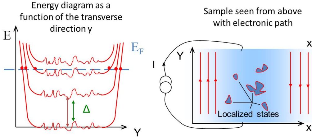
Figure 3.14: Schematic representation of disorder and localized states
