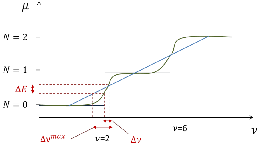
Figure 8.10: Filling factor as a function of the potential. The green curve sketches a realistic variation of \nu with \mu whereas the blue curve shows the linear variation used to compute a upper bound for \Delta n .
