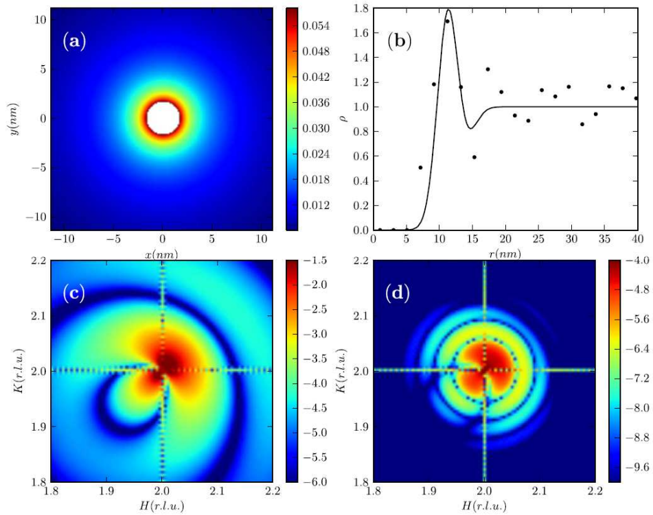
FIGURE 4.12: (a) Amplitude of the atoms radial displacements (in nm), following an isotropic elastic model around a cylindrical inclusion.(b) Radial pair distribution function of the nanocolumns, measured experimentally (dots) and fitted using a gaussian + error function model. (c) Scattering from a single isolated nanocolumn around the (220) reflection, including the scattering contributions from the displaced atoms as well as the missing atoms inside the column (see text for details). (d) Scattering of an assembly of nanocolumns around the (220) reflection, by taking into account their radial distribution function shown in (b). Intensity is plotted with a logarithmic color scale for (c-d).
