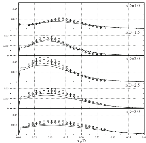
Figure 4.13: Re_D = 70000 test-case C3. Turbulent kinetic energy \frac{1}{2}(\langle u_s''u_s'' \rangle + \langle u_n''u_n'' \rangle)/U_b^2 : — , resolved fluctuations; - - , resolved fluctuations plus SGS contributions; \circ , HWA measurements [8].
