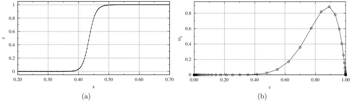
Figure 5.1: Mono-dimensional laminar flame test: progress variable c versus x (a); reaction rate \omega_c versus progress variable c (b). The flame speed was set at S_{L,\max} according to Eq. (5.24).
