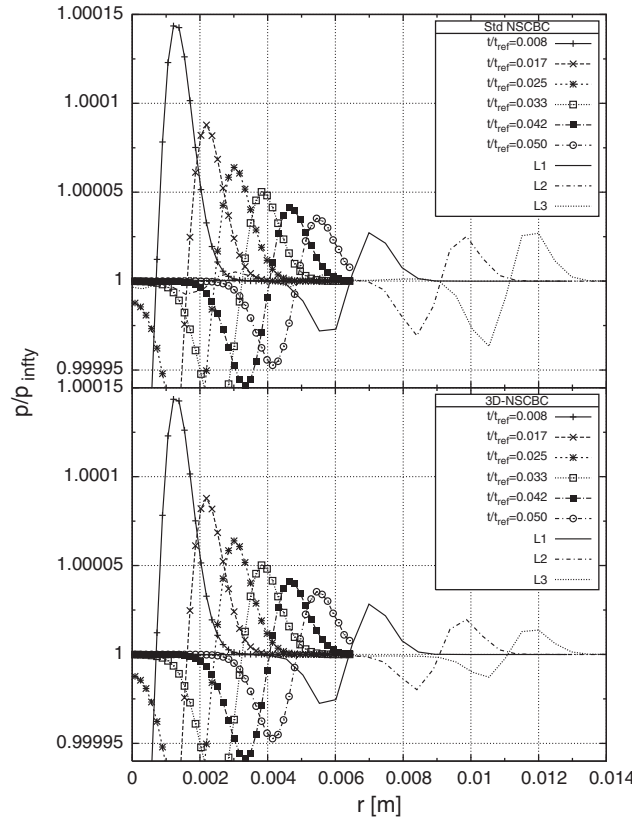
Fig. 17. Spherical pressure wave test: normalized pressure wave evolution r for test-case T3. Symbols are radial pressure plots at different normalized time-steps ( t_{ref} = 2.8 \times 10^{-4} s); lines are temporal pressure plots at locations L1, L2 and L3 rescaled as radial plots under the assumption that the pressure pulse is a signal traveling with speed c \simeq 347.6 m/s.
