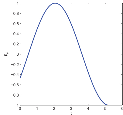
Figure 2.13: p_y for (2.27)–(2.29)
