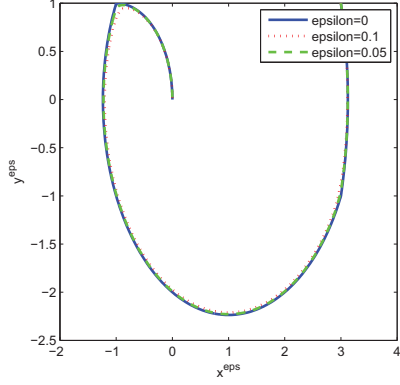
Figure 2.18: (x^\varepsilon, y^\varepsilon)
