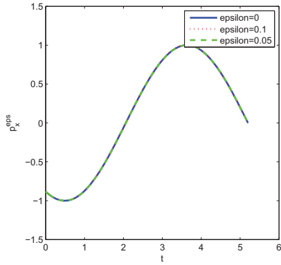
Figure 2.20: p_x^\varepsilon
