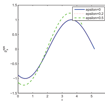
Figure 2.15: p_x^\varepsilon
