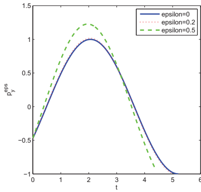
Figure 2.16: p_y^\varepsilon
