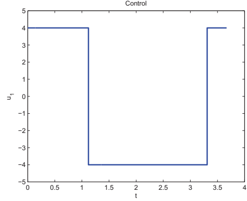
Figure 2.2: Optimal control
