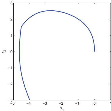
Figure 3.3: Optimal trajectory
