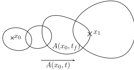
Figure 1.11: Minimal time.
