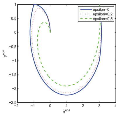
Figure 2.14: (x^\varepsilon, y^\varepsilon)
