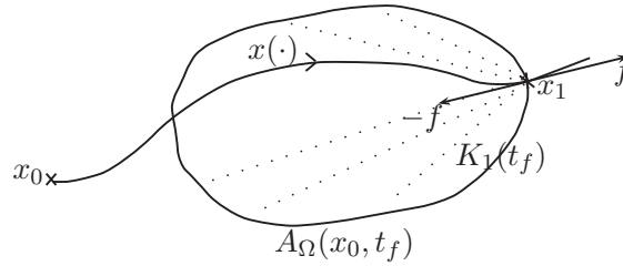
Figure 1.21: Cone K_1(t_f)
