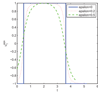
Figure 2.17: u_1^\varepsilon
