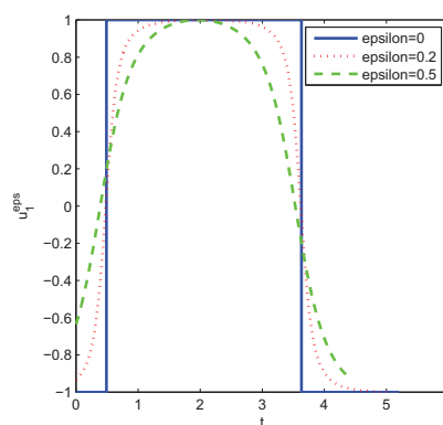
Figure 2.17: u_1^\varepsilon
