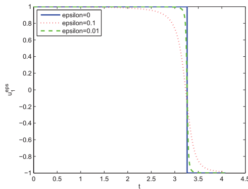
Figure 3.18: Control
