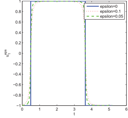
Figure 2.19: u_1^\varepsilon
