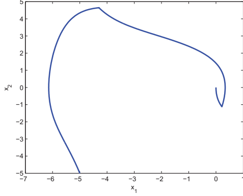
Figure 2.1: Optimal trajectory
