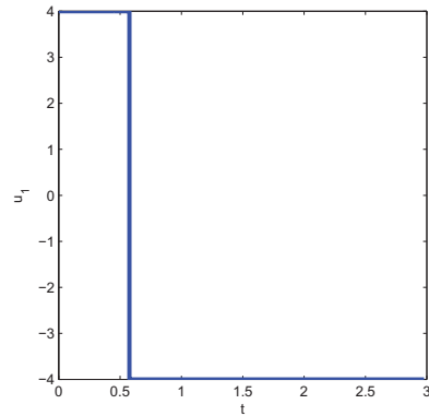
Figure 3.4: Optimal control
