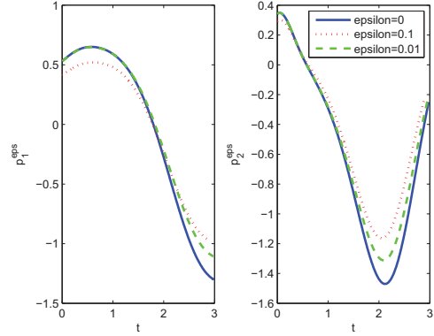
Figure 3.8: Adjoint vector
