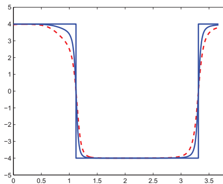
Figure 2.7: Control
