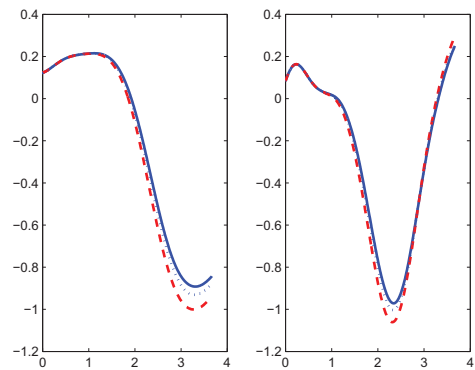
Figure 2.6: Adjoint vector
