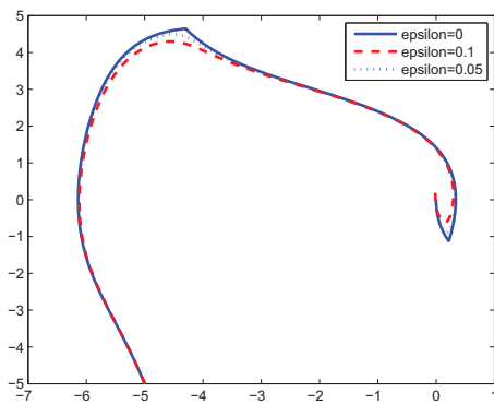
Figure 2.5: Trajectory
