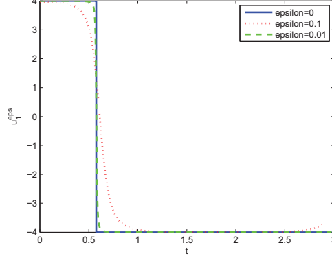
Figure 3.9: Control
