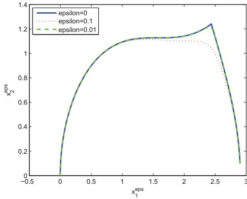
Figure 3.16: Trajectory
