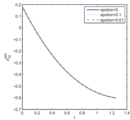
Figure 2.25: Adjoint vector p_{x_2}^\epsilon
