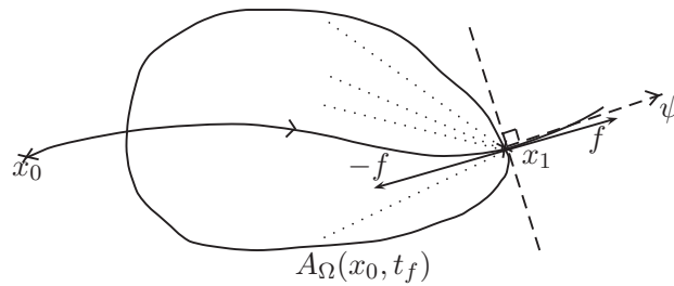
Figure 1.22: \langle \psi, f(x(t_f), u(t_f)) \rangle \geq 0
