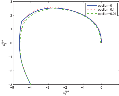
Figure 3.7: Trajectory
