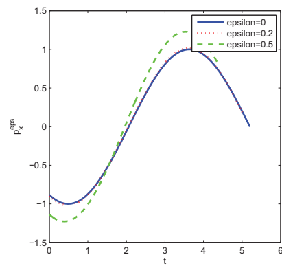
Figure 2.15: p_x^\varepsilon
