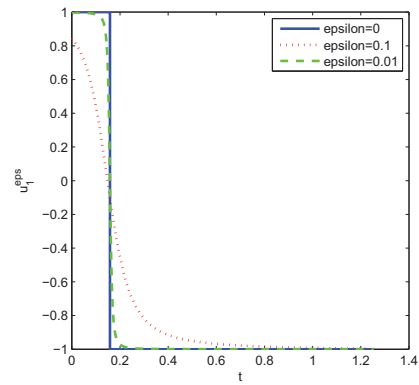
Figure 2.23: Control u_1^\epsilon(\cdot)
