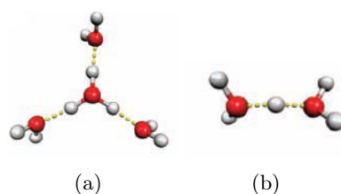
FIG. 3.3 – (a) Forme Eigen H_9O_4^+ (b) Forme Zundel H_5O_2^+ [65]
