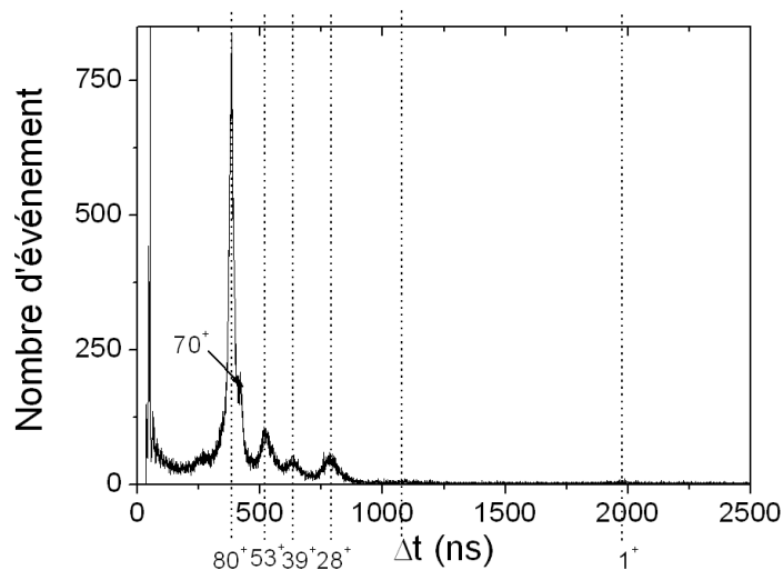
FIG. 3.54 – Spectre de fragmentation \text{Pyr}_2H^+
