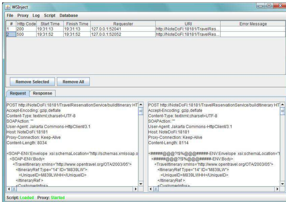
Figure 6.13: WSInject's GUI
