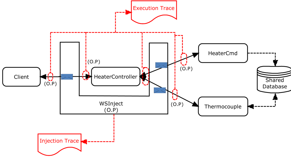
Figure 6.15: Testbed architecture of the heater controlling system
