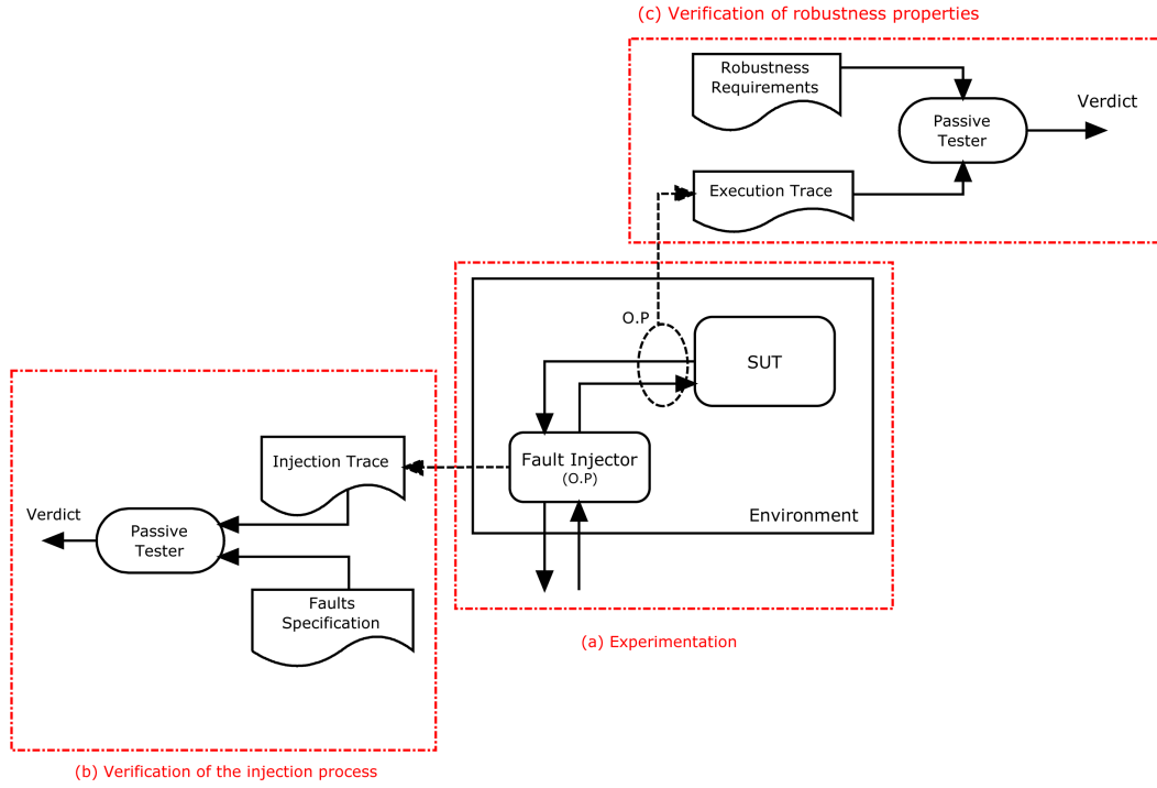
Figure 5.1: Architecture of the proposed robustness testing approach
