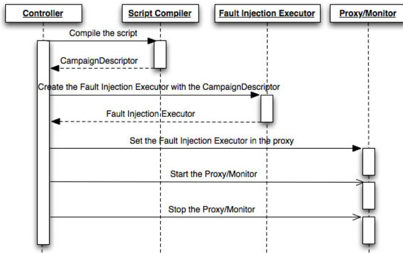
Figure 6.12: Initialization of WSInject's main components
