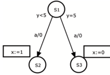
Figure 2.4: Information loss
