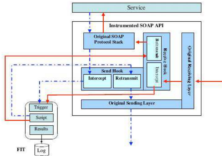
Figure 6.8: WS-FIT architecture
