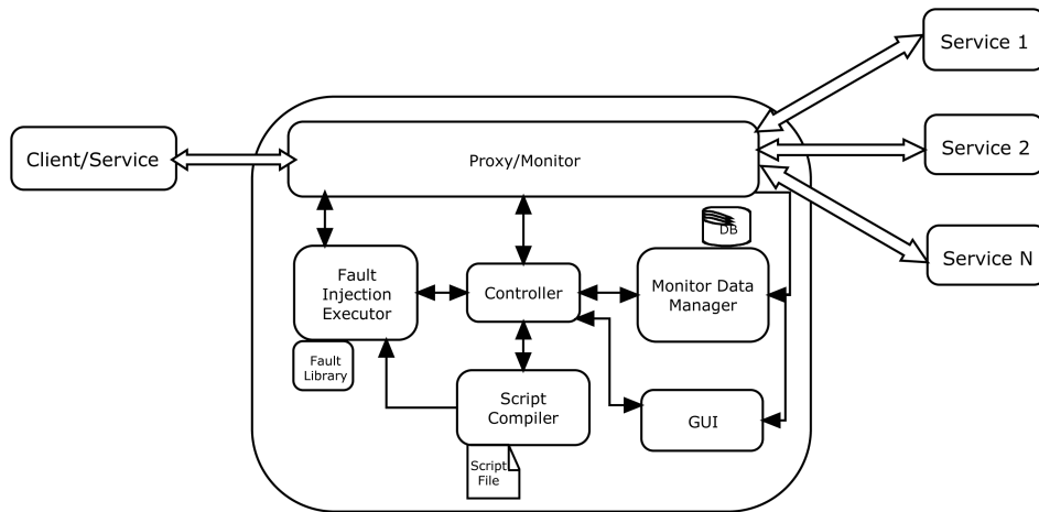
Figure 6.9: WSInject architecture
