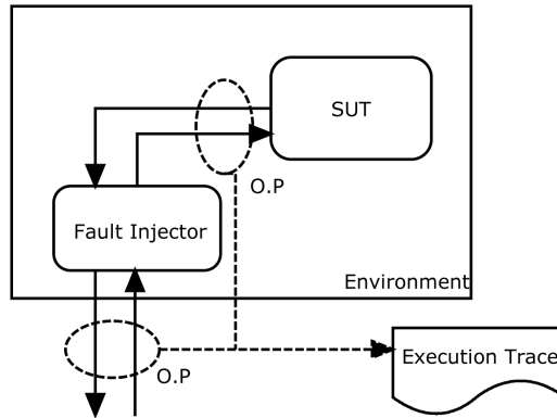
Figure 5.2: Observation points for distributed systems
