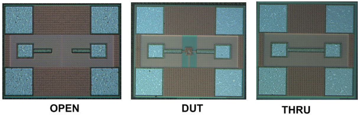
Figure A-3: Structures de de-embedding : OPEN-THRU et DUT.
