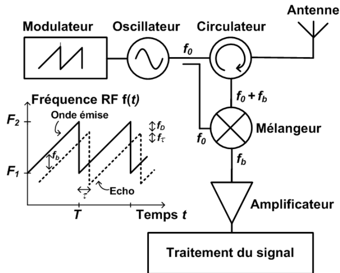
Figure I-12: Système radar FMCW.
