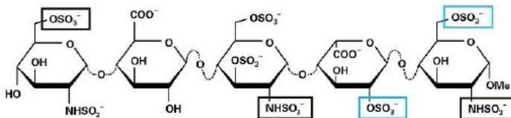
Figure 22: Sulfated and carboxylated carbohydrate-sequence of Fondaparinux , from (318) .
