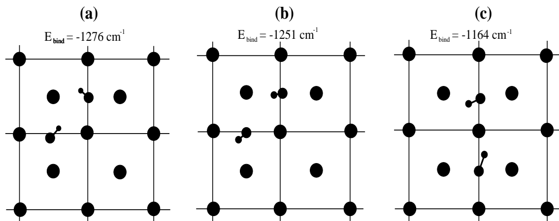
Figure 2.3: The energetically lowest adsorption geometries of two CO molecules adsorbed on Ar(100) (fcc). The adsorption energy E_{bind} is -1276 , -1251 and -1164 \text{ cm}^{-1} , respectively (from Parneix [61]).
