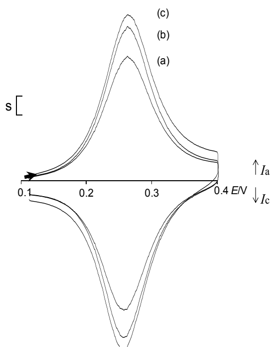
Figure 21. Cyclic voltammograms recorded ( 10 \text{ mV s}^{-1} in \text{CH}_3\text{CN} containing 0.1 M TBAP as supporting electrolyte) for C|poly2 modified electrodes synthesized using 4 \times 10^{-3} \text{ M} of monomer at + 0.85 V at different polymerization charges : (a) 1, (b) 2 and (c) 3 mC. S = 0.25 \text{ } \mu\text{A} .
