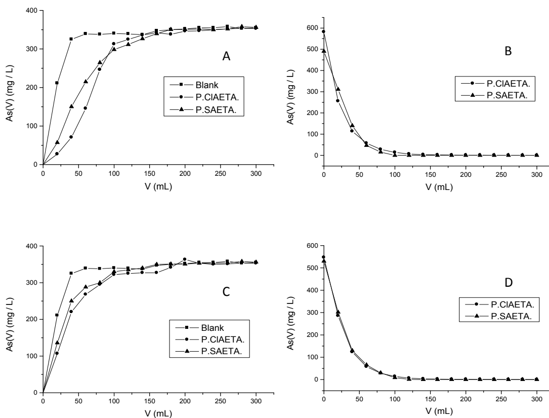
Figure 31. Charge-discharge process of arsenate ions using P(CIAETA) y P(SAETA). (A) first charge process of polymers through enrichment method at pH 8, (B) first discharge process of polymers using washing method at pH 3 with HCl 10^{-1} M. (C) recharge of polymers through enrichment method at pH 8, (D) second discharge process of polymers using washing method at pH 3 with HCl 10^{-1} M.
