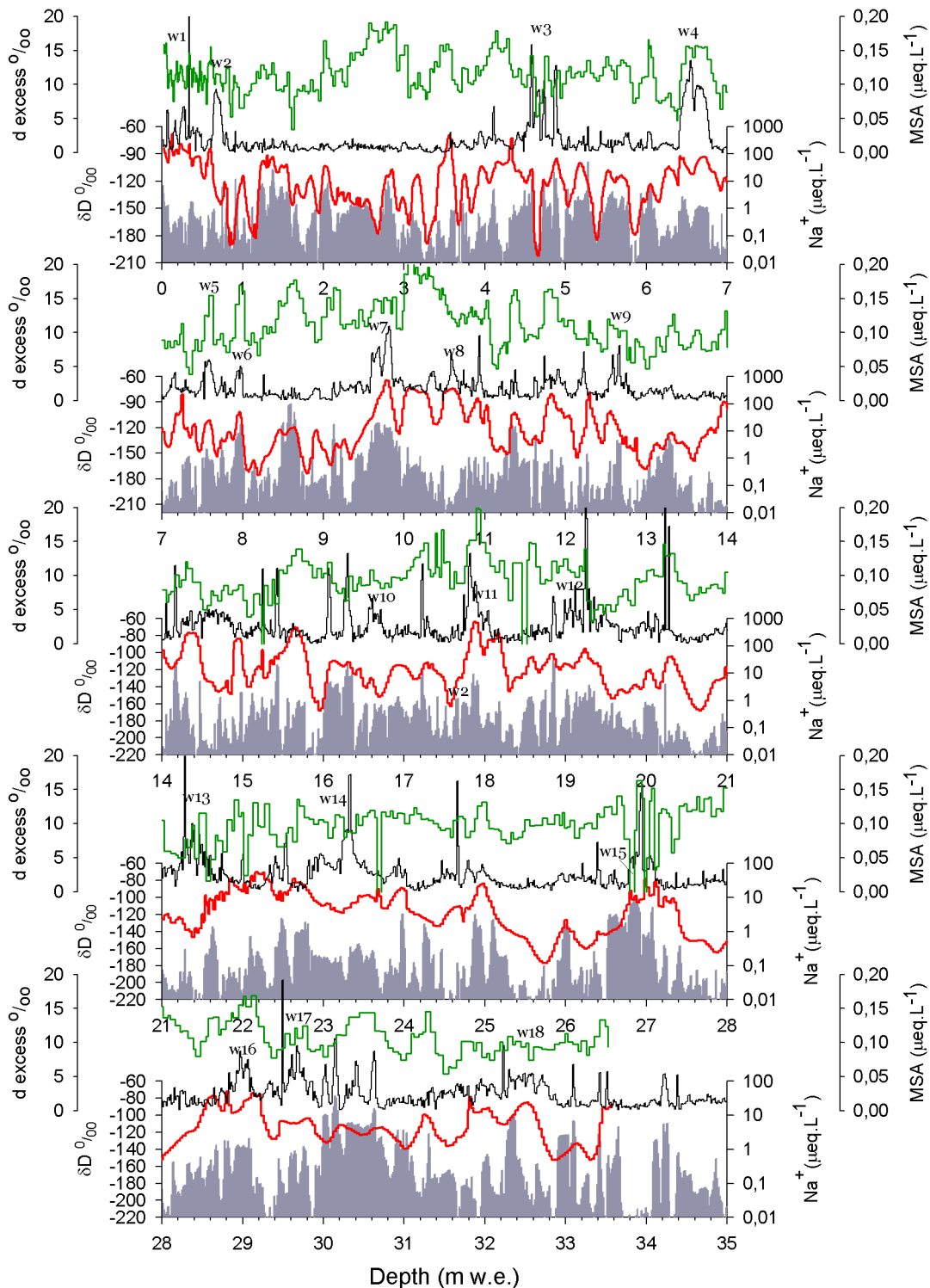
Figure 3.6: Deuterium excess (green, left-hand scale), \delta D (red, left-hand scale), \log Na^+ (shaded gray, right scale) and MSA^- (black, right scale) profiles for the first 33 m w.e. of the CL 122 core where fine resolution measurements of stable water isotopes are available. Isotopes measurements were made at the LAMA (Herreros, 2010). Wide peaks of MSA^- are numbered from w1 to w18 in this section of the core.
