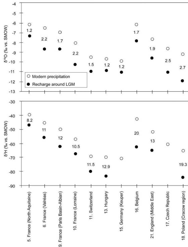
Fig.4. Contrasted isotopic content between LGM European groundwaters and modern precipitation. Numbers on the plots represent the difference between modern precipitation and LGM recharge. Data comes from references listed in Tab.1.
