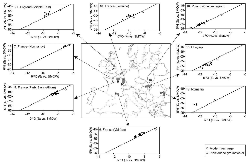
Fig.5. The \delta^2\text{H} and \delta^{18}\text{O} composition of Pleistocene groundwaters in Europe compared with the average of modern local precipitation and the GMWL. References and isotopic data listed in Tab.1.
