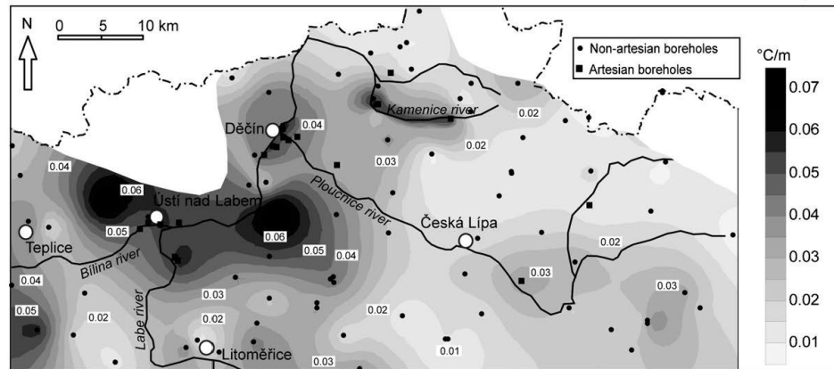
Fig. 7. Distribution of calculated geothermal gradients in the Benešov–Ústí aquifer system. The gradient calculation includes careful handling of vertical groundwater flow and the correction for the topography effect.
