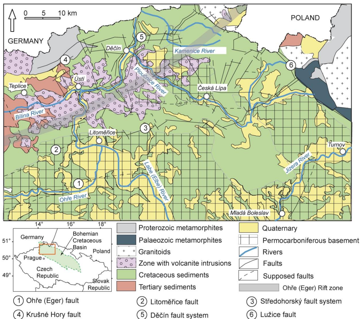
Fig. 3. Simplified schema of the study area in the Bohemian Cretaceous Basin showing main geological units and fault structures.
