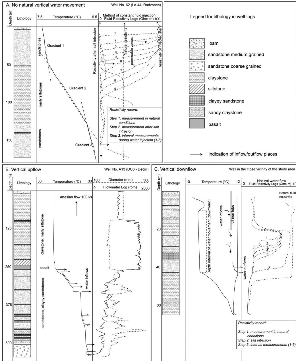
Fig. 5. Well-logs reflecting contrasted hydrodynamic conditions encountered within the study. The figure shows the registration and measurement heterogeneity in a well without vertical flow, with an upward vertical flow, and downward vertical flow. Inflow locations into the well are indicated by an arrow in the temperature column. (A) No vertical groundwater flow, geothermal gradients controlled by lithological properties, method of constant fluid injection has been used to assess the permeable zones, (B) upward groundwater flow (artesian well) and (C) downward groundwater flow typical for drainage and infiltration areas are reflected in the temperature log. Inflow sites are detected by resistivity measurements under natural conditions.
