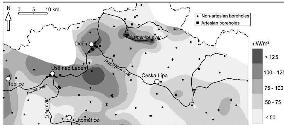
Fig. 8. Heat flux distribution in the Benešov–Ústí aquifer system as assessed from the geothermal gradients and the thermal conductivities of rock types. The map reveals generally higher heat flux in drainage zones in the western part, and lower values in the infiltration zones in the northeastern part of the study area.
