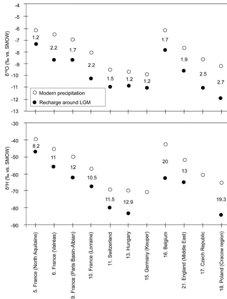
Fig. 4. Contrasted isotopic content between LGM European groundwaters and modern precipitation. Numbers on the plots represent the difference between modern precipitation and LGM recharge. Data comes from references listed in Tab. 1.
