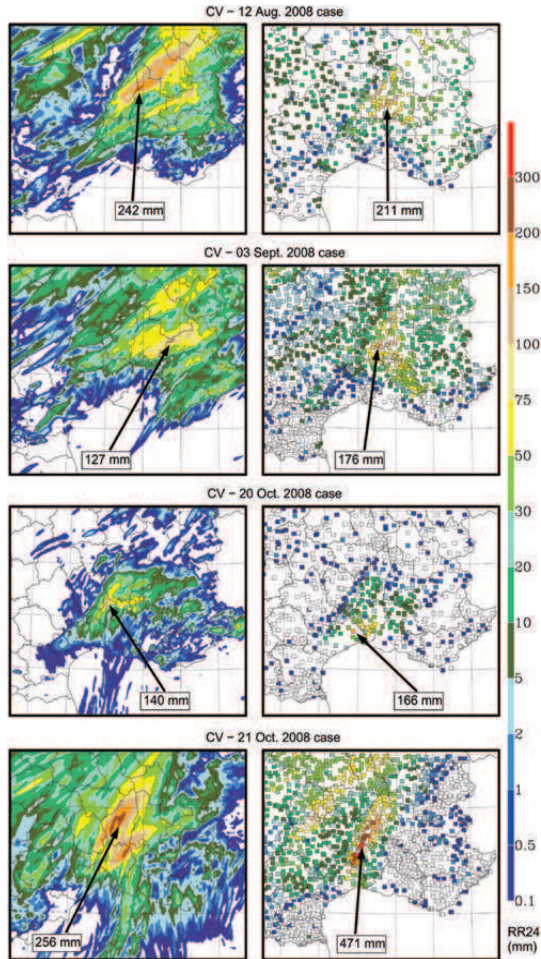
Fig. 3. 24-h accumulated precipitation ( \pi_{24} in mm) from the HRA2.5 simulations (left panels) and the Météo-France rain-gauge network (right panels) at 00:00 UTC, 13 August 2008 for the 12 August 2008 case (top), at 06:00 UTC, 4 September 2008 for the 3 September 2008 case (middle top), at 00:00 UTC, 21 October 2008 for the 20 October 2008 case (middle bottom) and at 06:00 UTC, 22 October 2008 for the 21 October 2008 case (bottom). The maximum of precipitation is indicated on each panel.
