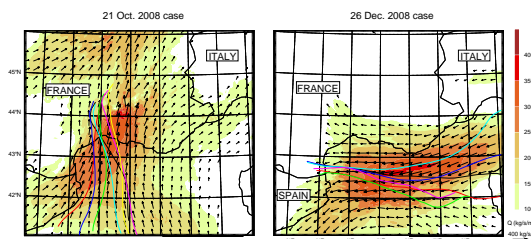
Fig. 11. HRA2.5 simulated water vapour flux Q integrated over the lowest 3000 m (in \text{kg s}^{-1} \text{m}^{-2} , colour scale on the right of the figure, and arrows) and horizontal projection of the backward trajectories of some air parcels taken in the precipitating systems simulated by HRA2.5 for the 21 October 2008 case (left) and the 26 December 2008 case (right). The arrows are drawn every 10 grid points with a scale given by the length of the arrow at the bottom right of the figure. Arrows are displayed only when corresponding to values of integrated water vapour flux larger than 80 \text{ kg s}^{-1} \text{m}^{-2} . The backward trajectories are the same as in Figs. 7 and 9. They show the parcel trajectories from 09:00 UTC till 19:00 UTC for the 21 October 2008 case and from 05:00 UTC till 15:00 UTC for the 26 December 2008 case. The background of the trajectory figure is a snapshot of the integrated water vapour flux at 14:00 UTC for the 21 October 2008 case and at 08:00 UTC for the 26 December 2008 case.
