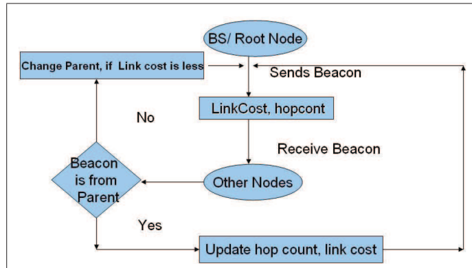
Figure 2.7: MultihopLQI
