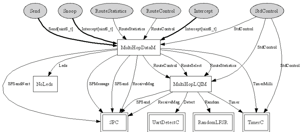
Figure 2.11: MultiHopRouter configuration. Direction of arrows indicates interface provider/user relationships NOT data flow direction.
