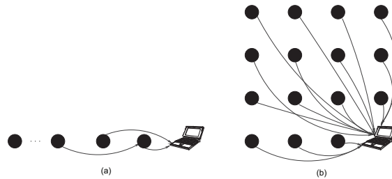
Figure 4.1: Straight-line (a) and Grid (b) deployment.
