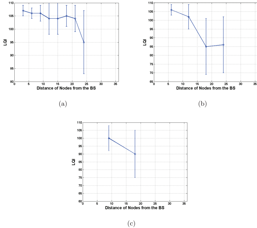
Figure 4.30: LQI of the Beacons Received from the BS, (a) Scenario 19 (b) Scenario 21 (c) Scenario 23. BS TPL= 10, node TPL =10
