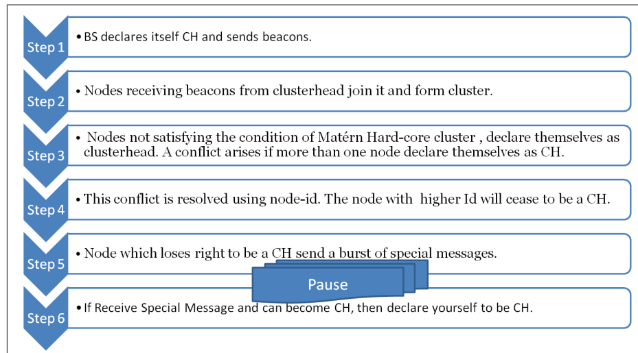
Figure 7.5: Matérn Algorithm
