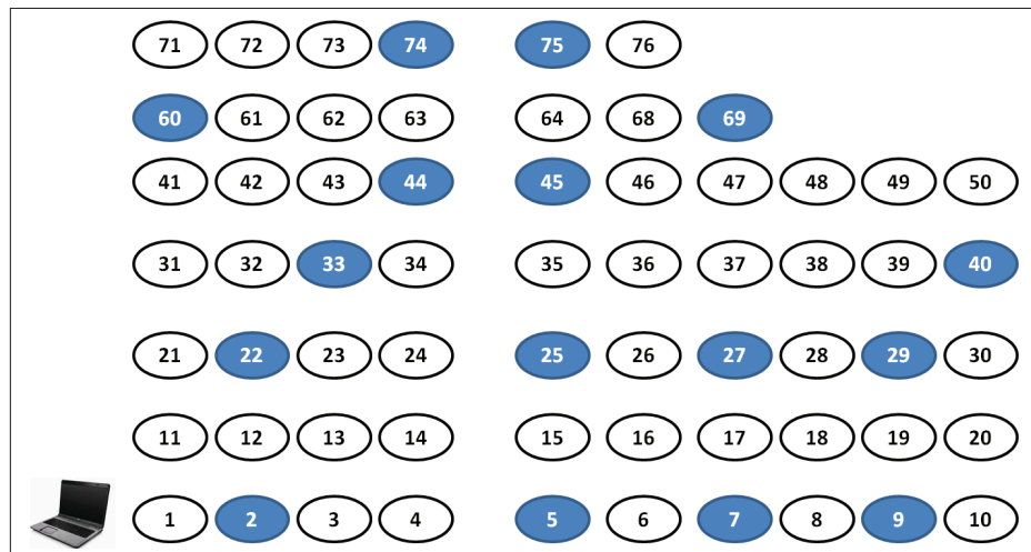
Figure 7.17: Output of Matérn Hardcore Process in grid topology
