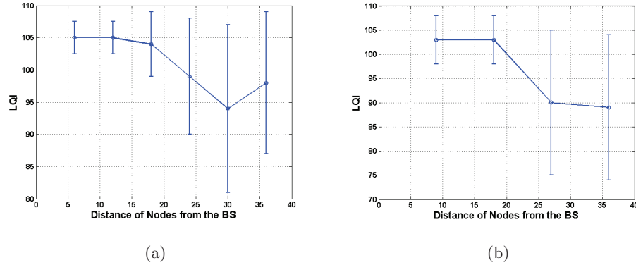
Figure 4.31: LQI of the Beacons Received from the BS, (a) Scenario 20 (b) Scenario 22. BS TPL= 31, node TPL =10
