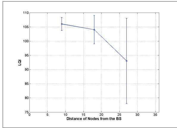
Figure 4.10: Scenario-4, LQI of the Beacons Received from the BS, BS TPL=25, node TPL=25
