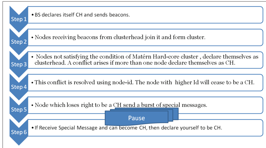
Figure 7.5: Matérn Algorithm
