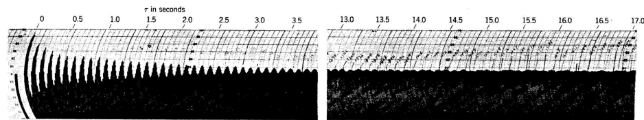
AUTOCORRELATION
