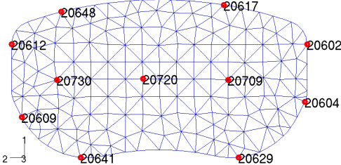
Figure 4.55: Selected pad nodes for the following phase plots. The disc is moving from left to right. Contact normal direction 3, contact plane, directions 1 and 2
