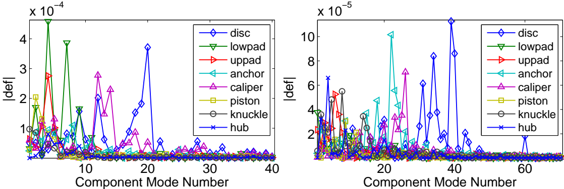
Figure 5.39: Projection of the principal shapes given by the SVD on the component modes through the component mode model. Left: SVD singular shape #1. Right: SVD singular shape #2
