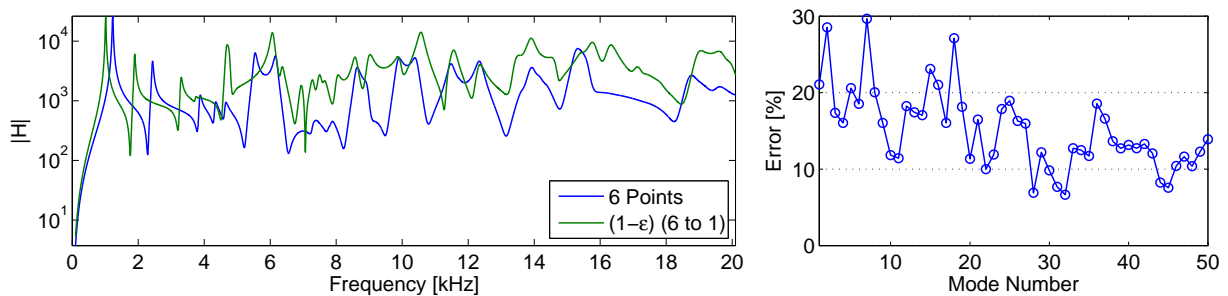
Figure 2.54: Left: Dynamic behavior differences between the use of a 6 point integration rule contact integration law, and the regularization strategy based on a 1 point integration rule for \epsilon = 10^{-3} (42% of quasi-compatible shapes kept). Right: Frequency differences observed at peaks
