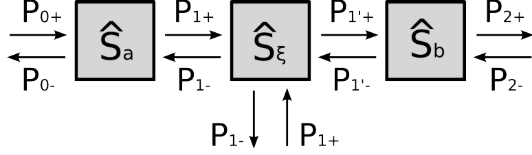
Figure 3.3: Cartoon of the system in presence of the voltage probe.
