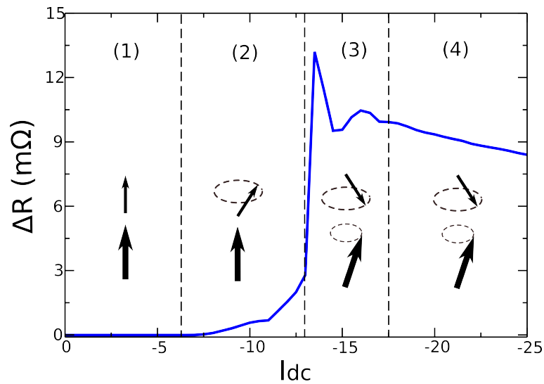
Figure 6.23: Resistance as a function of current calculated for H_{\text{ext}} = 11 KOe. Resistance varies sensitively from one region to the other, with the steepest variation in region (3), when reversal occurs.
