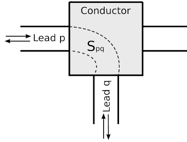
Figure 2.6: Scattering matrix that connects leads p and q in a multi-terminal device. In such a device, each pair of leads has its own scattering matrix that describe transport properties
