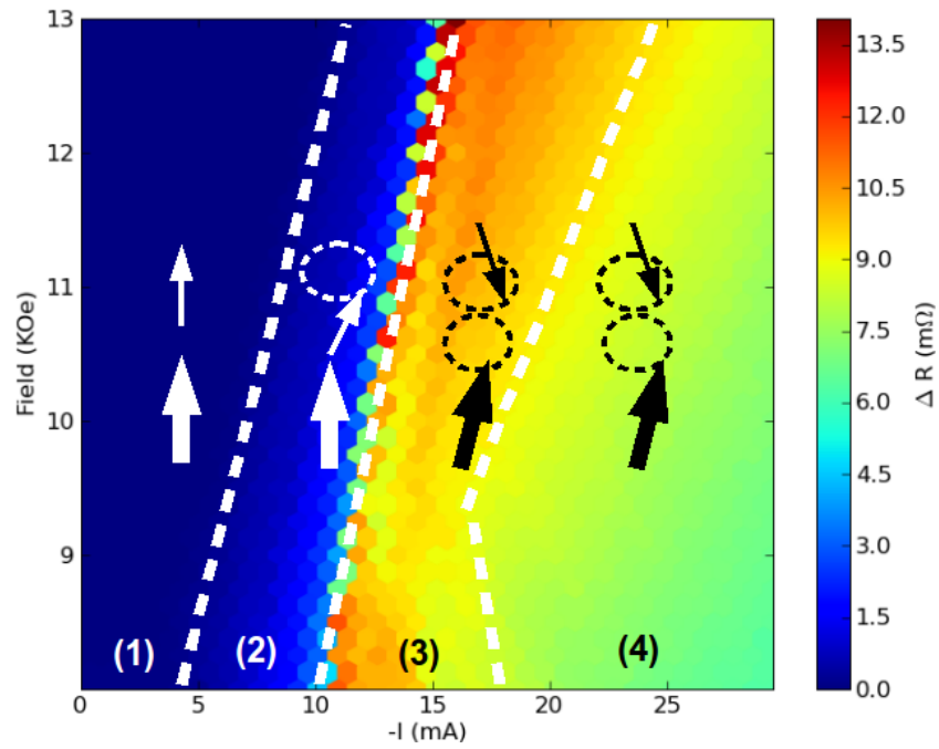
Figure 6.21: Simulated phase diagram of the resistance as a function of current and magnetic field. The diagram is divided in 4 regions with different dynamics. Region (1): both the layers are aligned with \hat{e}_z ; region (2): precession of the thin layer; regions (3) and (4): magnetization reversal and precession of both layers (see text).
