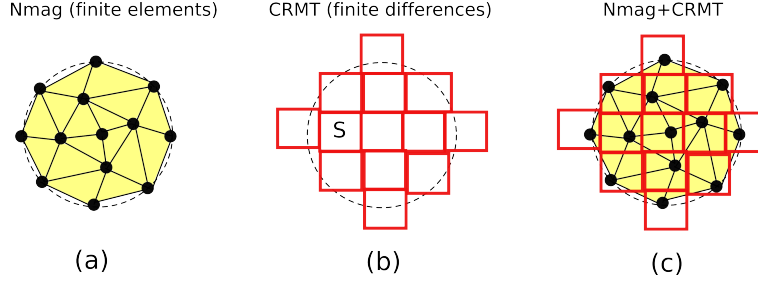
Figure 6.13: Different simplified representation of our system. In fig. (a) the disk is discretized using finite elements where each dot consists in a site i with magnetization \hat{e}_{Mi} , connected to the other sites through an irregular mesh. In fig. (b) the same disk is discretized using finite differences, as an assembly of pillars (represented by red squares) connected in parallel, each one with the same cross section S . Fig. (c): each CRMT pillar contains one site lying at the surface. See text for details about the coupling between CRMT and finite element representation.
