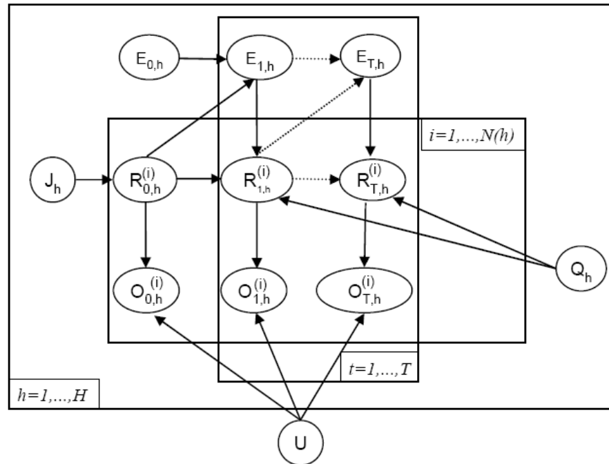
Figure 2.5. Network describing the temporal evolution of individual health states of animals within an infected dairy cattle herd. R_{t,h}^{(i)} \in \{S, I-, I+, R\} represents the real and non-observed health state of individual i belonging to herd h ( i \in \{1, \dots, N(h)\} ) with N(h) the total number of cows in the herd h , h \in \{1, \dots, H\} and H the number of herds) at time t ( t \in \{0, \dots, T\} ) with t=28=T and t=0=0 ). E_{t,h} describes the quantity of bacteria in the environment of the herd h at time t . O_{t,h}^{(i)} represents the observed health state associated with R_{t,h}^{(i)} . J_h is the probability distribution of the initial real health states and U is the matrix of the uncertainty parameters ( Se and Sp of tests) linking real and observed health states. Q_h contains the parameters of transitions between real health states in herd h except those characterising the S \rightarrow I- transitions. Q_h is a 3 \times 4 matrix corresponding to the last three rows of matrix Q_{t,h} described in Equation (3.1).
