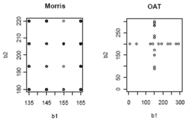
Figure 3.3. Space sampling in grid for Morris OAT and in cross for standard OAT; b1 and b2 are two inputs factors.
