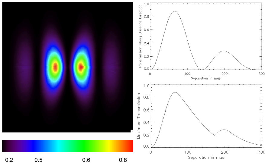
FIG. 1.— Left: PFN sky transmission over 0.6'' \times 0.6'' field of view, assuming a "horizontal" 3.20 m baseline separating two elliptical sub-apertures ( 3 \text{ m} \times 1.5 \text{ m} ). Top right: PFN transmission vs separation, along baseline direction. Bottom right: Maximum transmission versus baseline rotation angle, as a function of separation.
