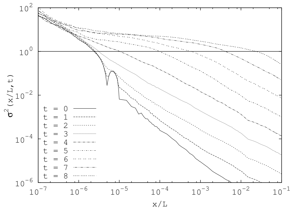
Figure 4.10: Evolution of the mass variance in the static case starting with an initial PS P_{init}(k) \propto k^0 at t_s = 0, 1, 2, 3, 4, 5, 6, 7, 8 . The x -axis is normalized by the box size.
