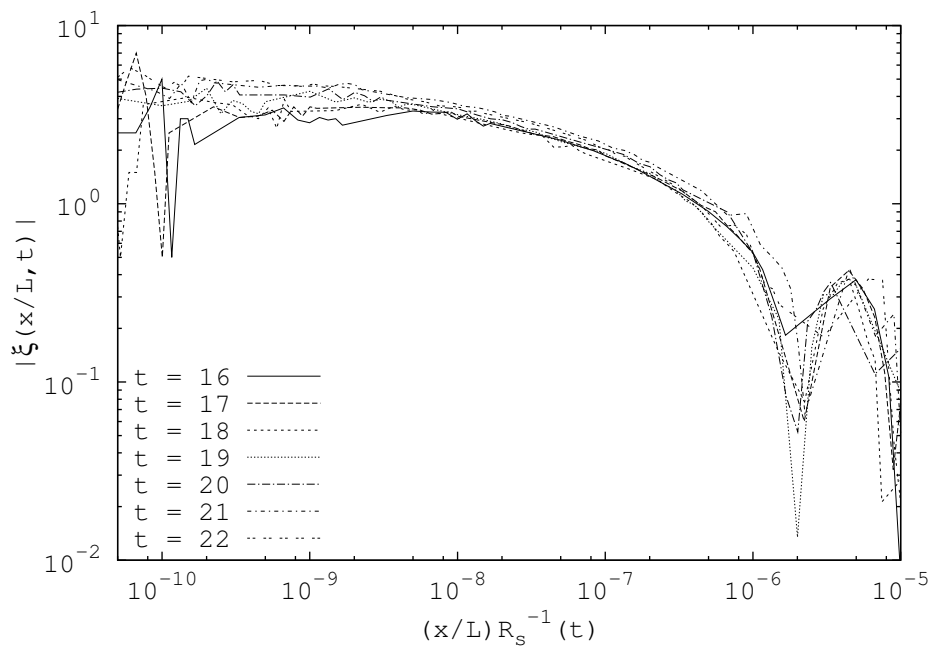
Figure 4.45: Temporal evolution of the correlation function as a function of x/R_s(t) , starting with an initial PS P_{init}(k) \propto k^4 for the static model at time t_s = 16, 17, 18, 19, 20, 21, 22 .
