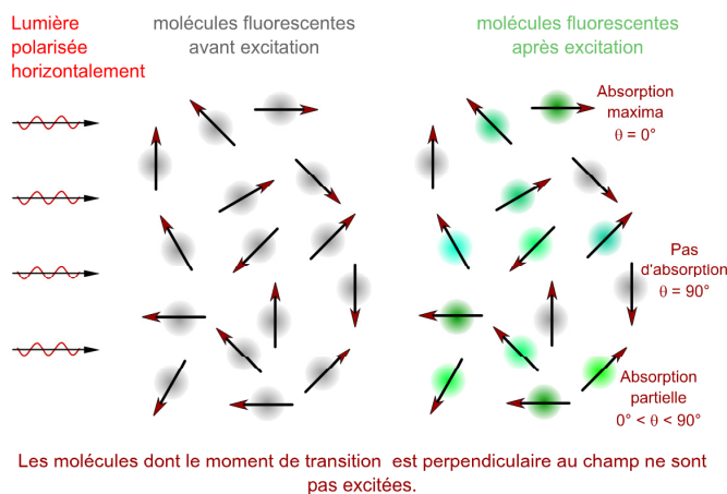
FIGURE 42 – Photoselection [52].
