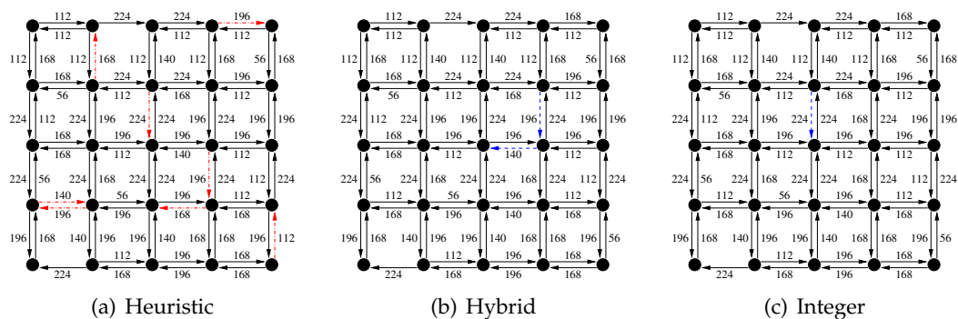
Figure 4.12: Very similar solutions (Grid 5 \times 5 , \lambda = 1.30 ).
