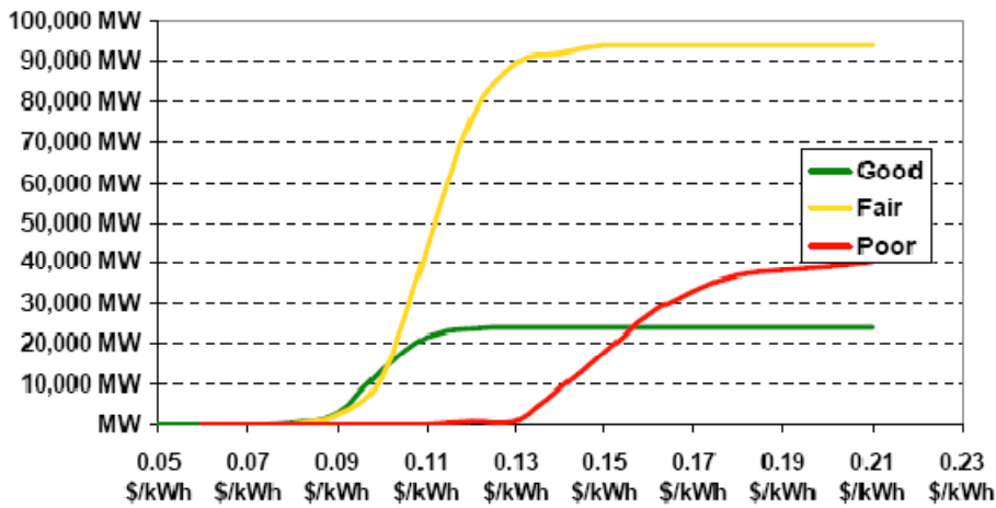
Figure 3-6: Potential new capacity of wind power in dependence of LECs.
