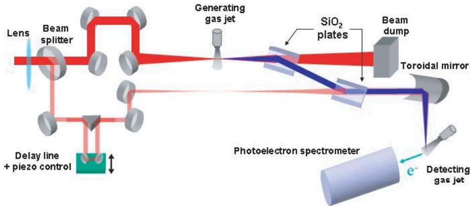
Fig. 1. (Color online) Principal sketch of the experimental set-up. The initial IR laser beam splits into pump and probe branch. The nonlinear interaction of the IR laser in the pump branch with the N_2 molecular jet drives the harmonics production. The harmonics are reflected and refocused into the interaction volume of a MBES, where they produce photo ionisation in argon. Temporal overlap of harmonic pulse and IR probe leads to the appearance of sidebands in the photoelectron energy spectrum.
