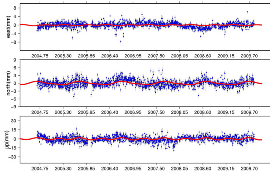
MSEL_GPS
