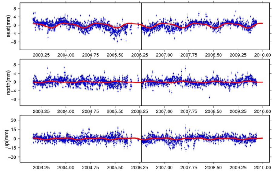
UNPG_GPS
