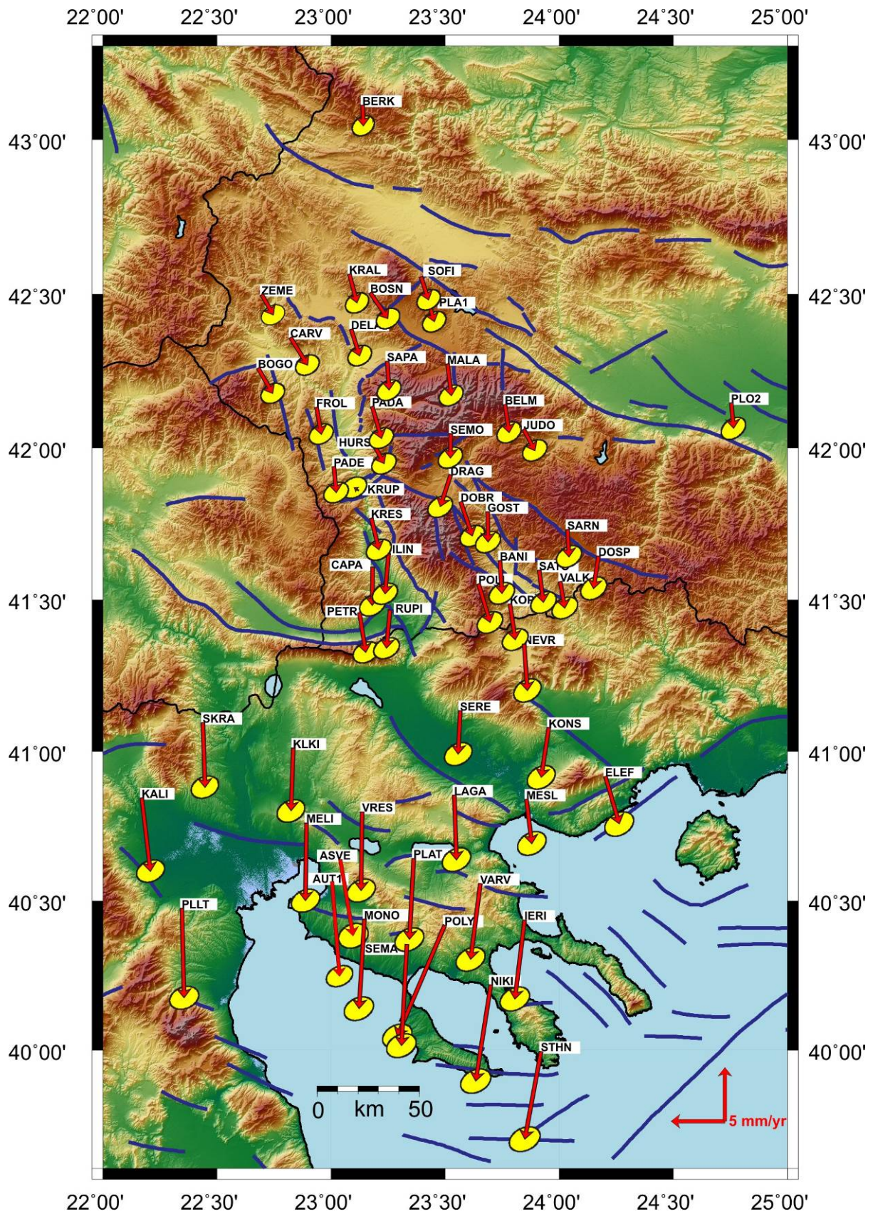
Figure 5.6. GPS velocities referred to stable Eurasia with their 3\sigma error ellipses for SWB and NG region.
