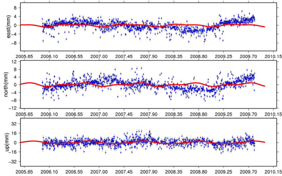
MRLC_GPS
