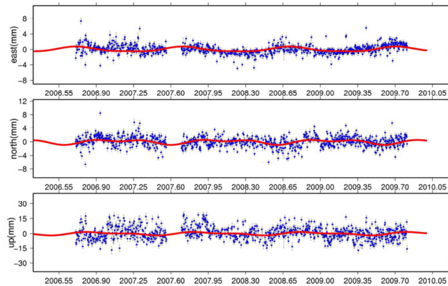
FRES_GPS
