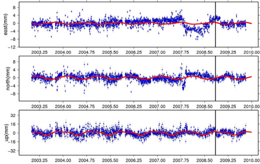
ORID_GPS
