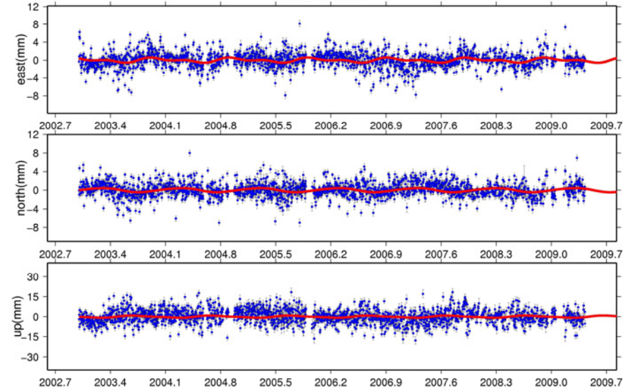
ELBA_GPS
