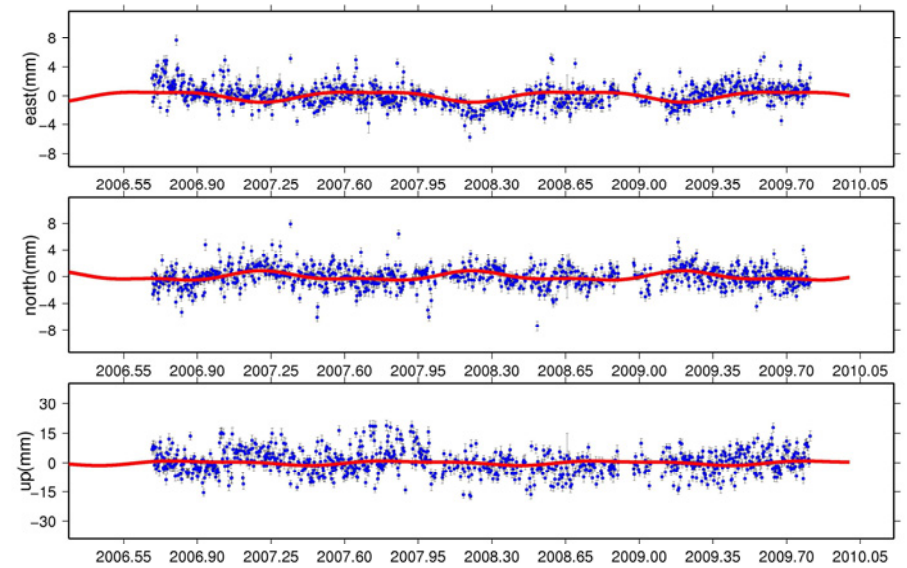
MRGE_GPS
