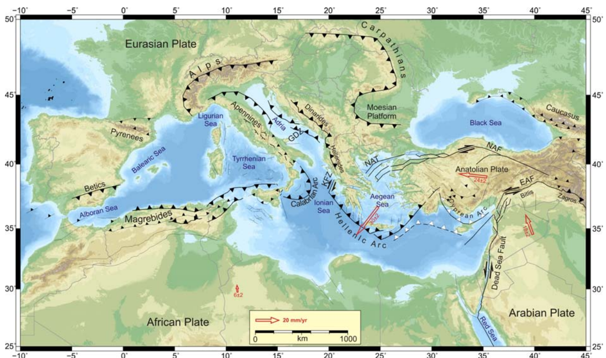
Figure 2.1. Geodynamic framework of the Mediterranean region. The major tectonic structures are adopted from Hollenstein 2006. The arrows represent plate motion relative to Eurasia (McClusky et al., 2000). NAF: North Anatolian Fault; EAF: East Aegean Fault; NAT: North Aegean Trough; KFZ: Kefalonia Fault Zone; GDZ: Gargano–Dubrovnik zone;
