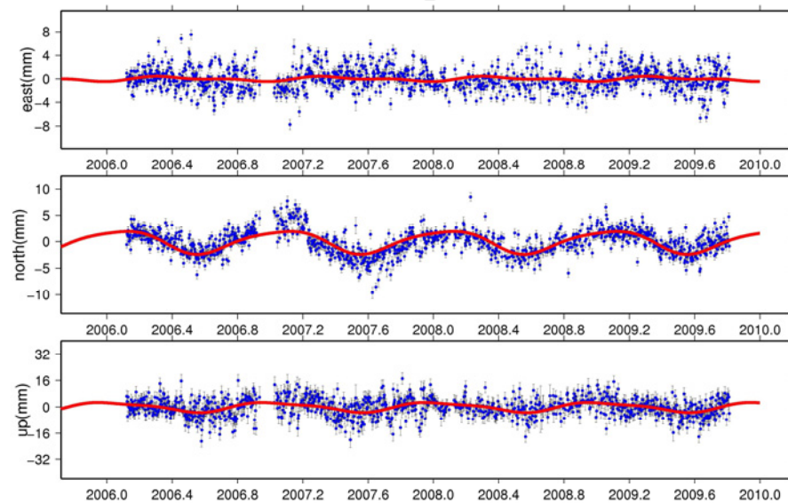
VLSM_GPS
