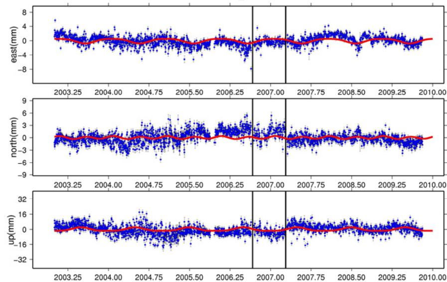
WROC_GPS
