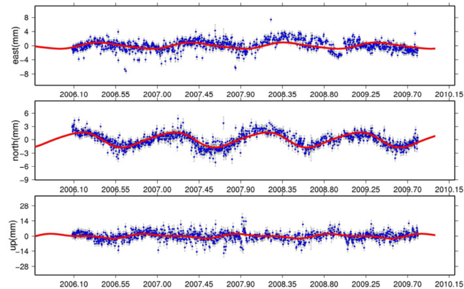
COST_GPS
