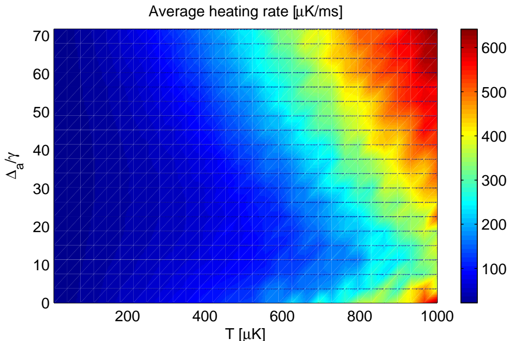
Figure 1.6: Average heating rate induced by detection light. Parameters are n_0 = 2.5 \times 10^{-2} , g_0 = 2\pi \times 160 \text{ MHz} , \Delta_c = 0 , U_{dip} = k_b \times 2.6 \text{ mK} , \Delta_{LS,0} = 2U_{dip}/\hbar = 2\pi \times 110 \text{ MHz} .
