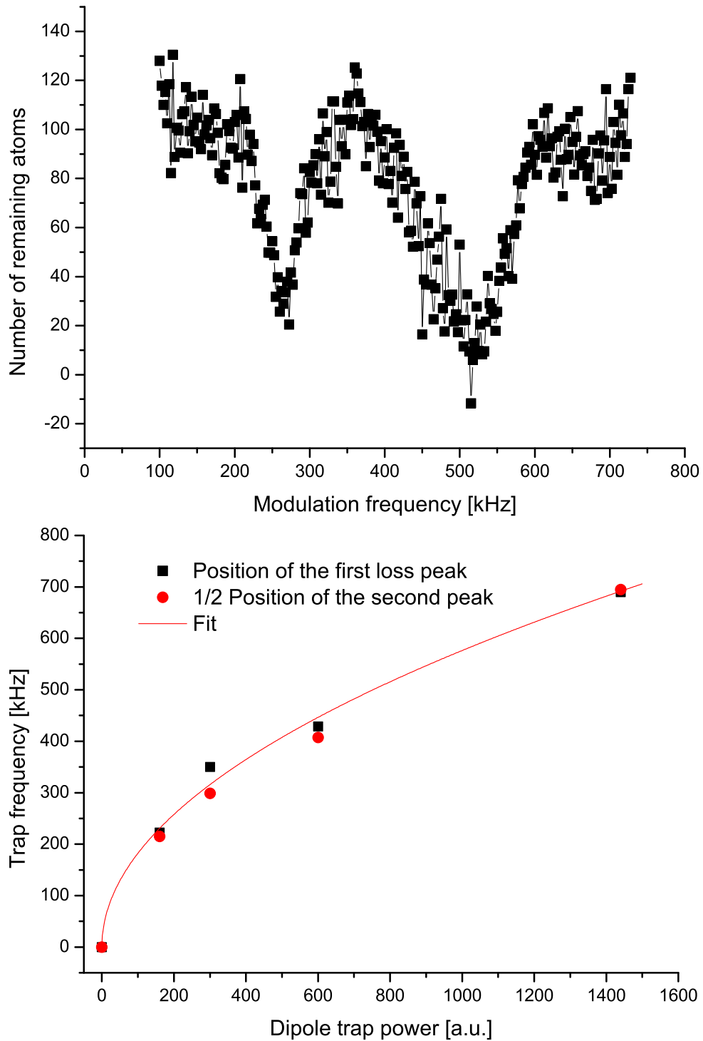
Figure 2.9: Calibration of the dipole trap frequency f_y . Top: Remaining atoms as a function of trap modulation frequency f_{mod} . Bottom: Modulation frequency for the two loss peaks, for different dipole trap depths. The frequency of the second peak is divided by two. The full line is a square-root fit.
