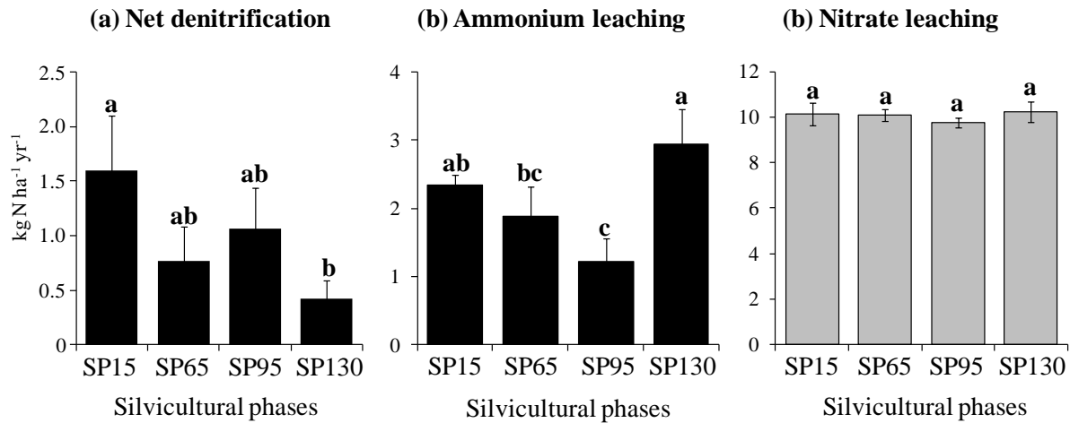
Figure 3.8. (a) Field net denitrification and (b) mineral N leaching (with root uptake) expressed as kg N ha -1 yr -1 according to silvicultural phases. Bars are standard errors and letters (a, b and c) indicate significant differences according to Kruskal-Wallis test at P < 0.05 ( n=4 ).
