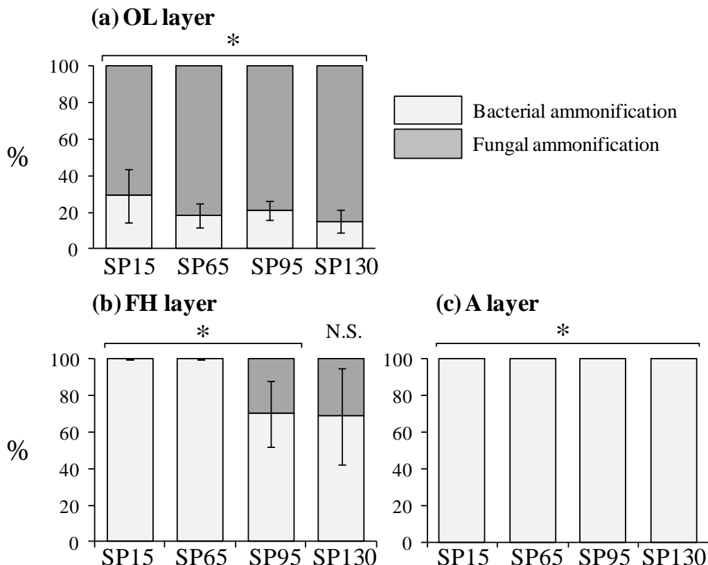
Figure 2.1. Net ammonification pathways, i.e. bacterial and fungal, within the OL (a), the FH (b) and the A layers (c) expressed as % of contribution in total net ammonium production according to silvicultural phases. Vertical bars correspond to standard deviation. "*" indicates significant differences at P < 0.05 between bacterial and fungal contributions while "N.S." refers to non significant (Wilcoxon rank sum test, n=4 ).
