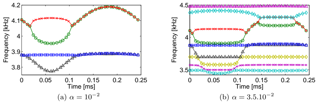
Figure 3.29: Frequency evolution of modes around mode C44 (4.2kHz) over an oscillation based on mode C44 pseudo cycle
