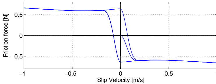
Figure D.3: Behavior of the LuGre model
