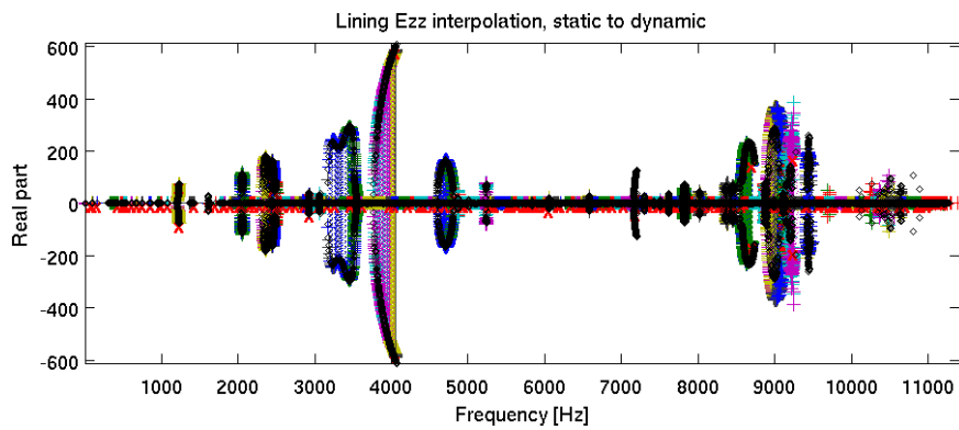
Figure 2.36: Stability diagram as function of the lining transverse Young modulus. (+) makers stand for the high E_{zz} value, ( \diamond ) for the low value used in the reduction basis
