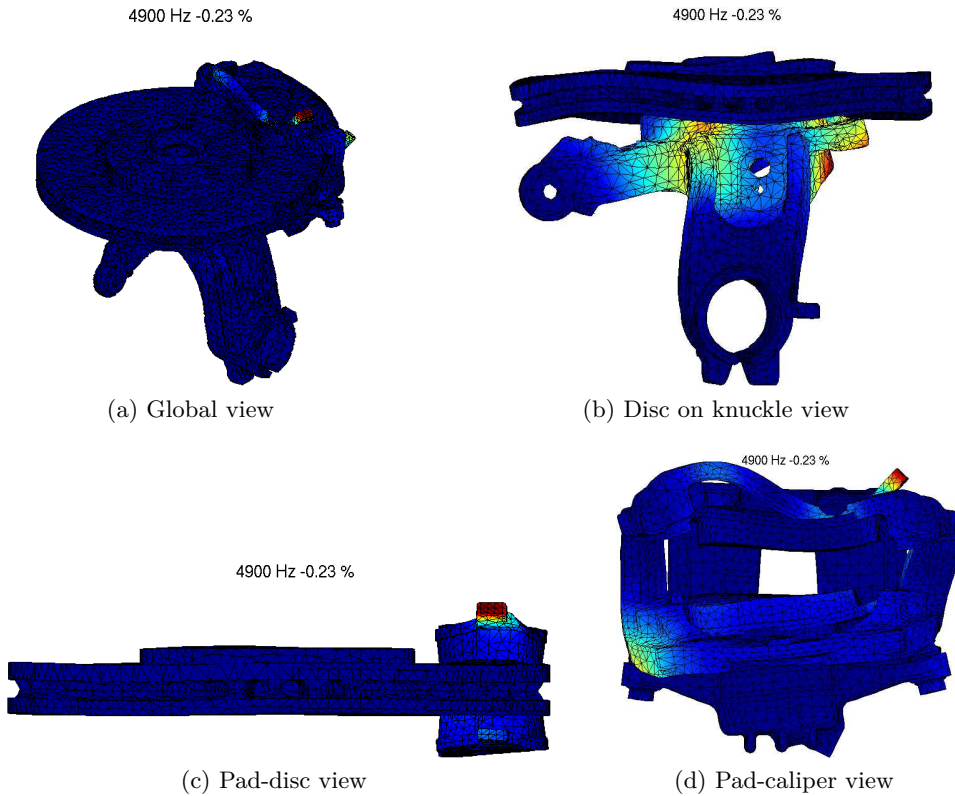
Figure 3.18: Mode C51 shape, colors are re-scaled for each sub-component view
