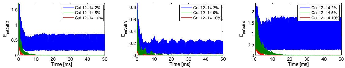
Figure 5.59: Effect of damping caliper modes 12 to 14 on the limit cycle obtained at 12 Bar, modal mechanical energy associated to caliper modes 12, 13 and 14
