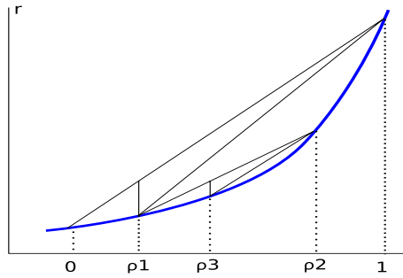
Figure 4.14: Illustration of the secant method for the line search algorithm
