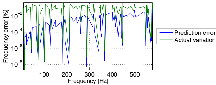
Figure 2.25: Prediction frequency error against recomputed frequency shift for a 0.1 gram increase on the half-plate #2 node #1
