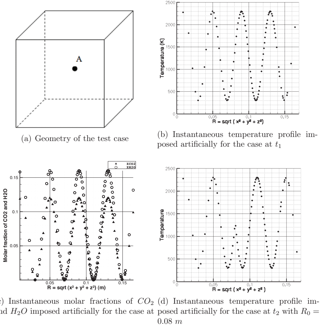
Figure 4.25 – Presentation of the test case to validate NIFI model
