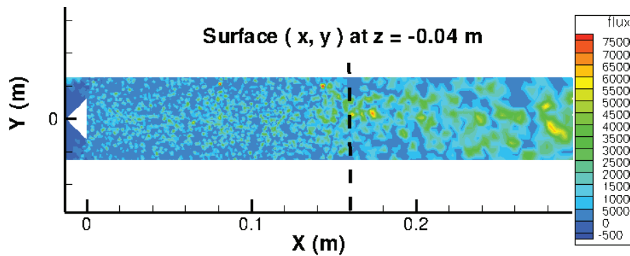
Figure 6.4 – Instantaneous radiative flux, in plan z = -0.04\text{ m} , \varepsilon = 1.0 , T_{wall} = 300\text{ K}
