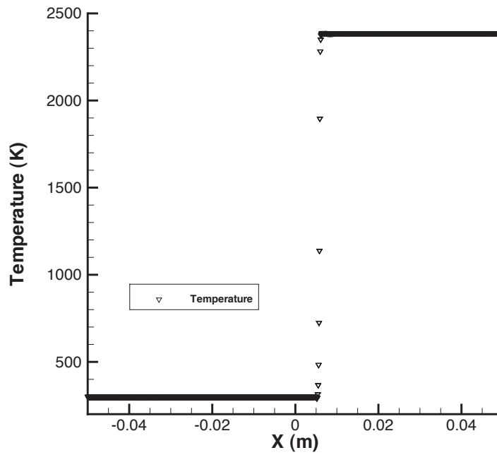
(a) Temperature
