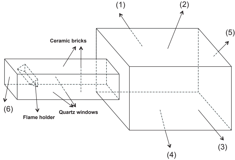
Figure 5.3 – Boundary conditions of "diedre_3d"
