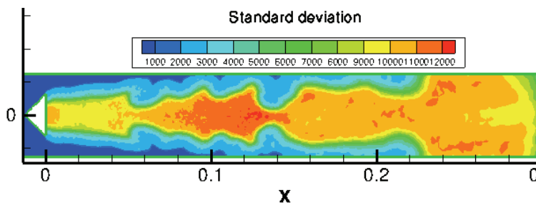
Figure 5.10 – Cut at z = -0.002 m of the standard deviation field (unit: W/m^3 ), converged result of Monte Carlo Method, "diedre_3d"
