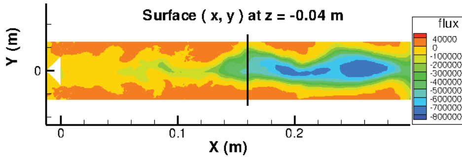
Figure 6.10 – Instantaneous radiative flux, in plan z = -0.04 \text{ m} , \varepsilon = 1.0 , T_{wall} = T_F \text{ K}
