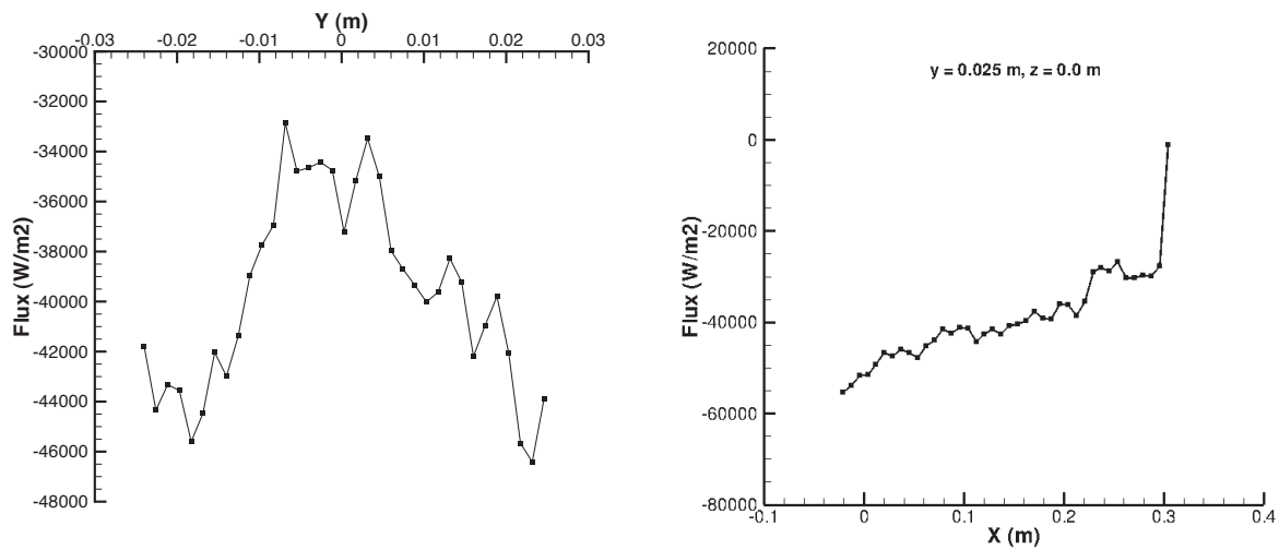
(a) surface (x,y) at z = -0.04 m and x = 0.16 m (b) surface (x,z) at y = 0.025 m and z = 0.0 m
