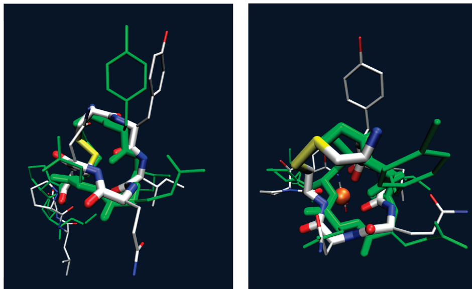
Figure 5. C_{\alpha} -based superposition of the OT X-ray structure (green, PDB code: 1NPO) with the calculated structure I of [\text{OT} + 2\text{H}]^{2+} (left) and structure II of [\text{OT} + \text{Cu}]^{2+} (right), in which standard colors for atoms have been used (N, blue; O, red; S, yellow; C, white). Thicker lines label bonds building the 20-member OT ring.
