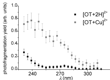
Figure 4. Experimental fragmentation yields of [\text{OT} + 2\text{H}]^{2+} and [\text{OT} + \text{Cu}]^{2+} ions measured as a function of the laser wavelength.
