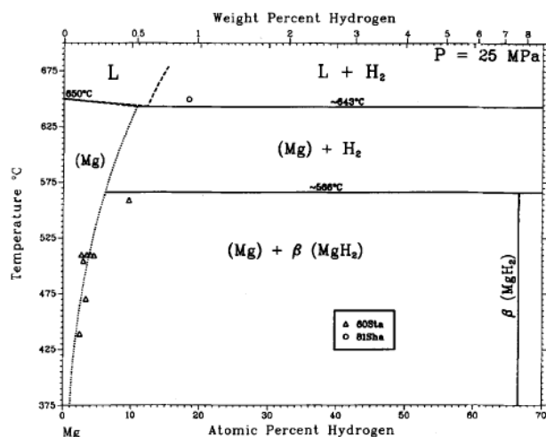
Figure 1.4. Assessed Mg-H phase diagram [26]
