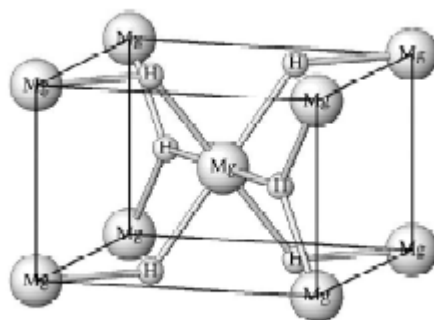
Figure 1.2. Crystal structure of \beta - MgH_2 (rutile type)
