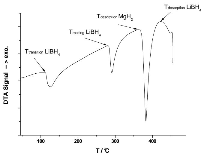
Figure 3.18. Thermal analysis of the hydride mixture ( x = 2 ) by DTA
