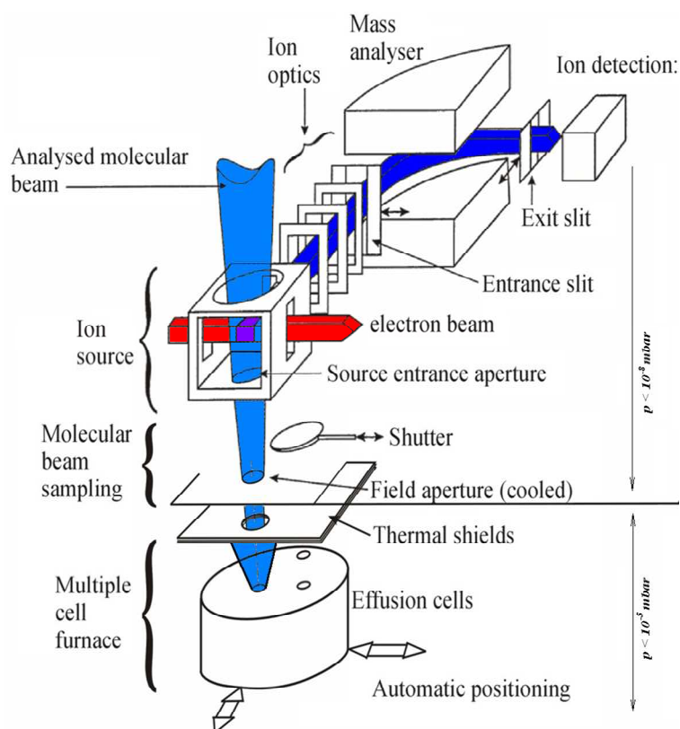
Figure 2.3. General view on the machinery of the mass spectrometer of SIMaP laboratory
