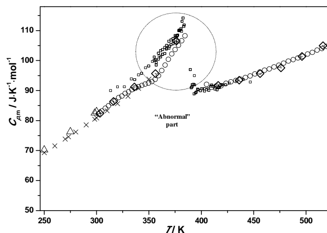
Figure 4.4. Experimental heat capacity data of \text{LiBH}_4 compound. - Low- T : \Delta , Nernst calorimetry [6]; \times , Adiabatic calorimetry [3]. - High- T : \square , DSC [3]; \circ , linear ramp and \diamond , enthalpy methods [this work].
