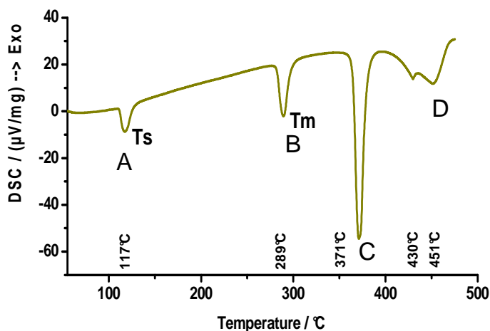
Figure 3.9. DSC curve of \text{MgH}_2\text{-2LiBH}_4 hydride mixture (Ar flow 100 \text{ ml}\cdot\text{min}^{-1} , 5 \text{ K}\cdot\text{min}^{-1} heating rate)
