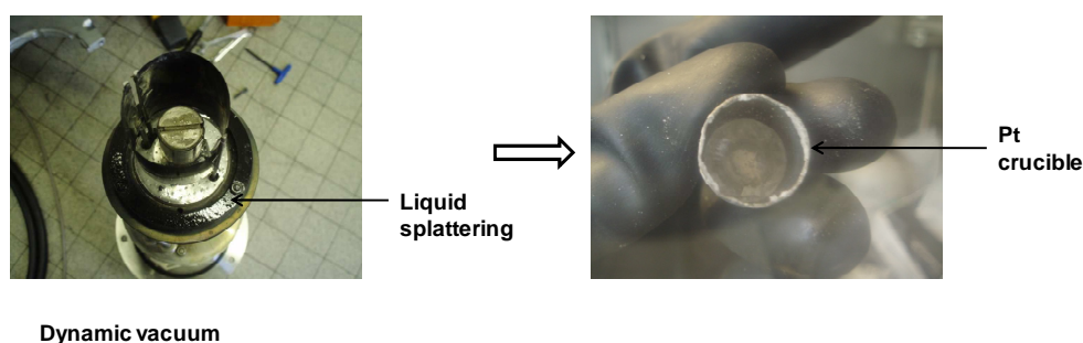
Figure 5.8. Liquid \text{LiBH}_4 evaporation tentative using high- T reactor under dynamic vacuum
