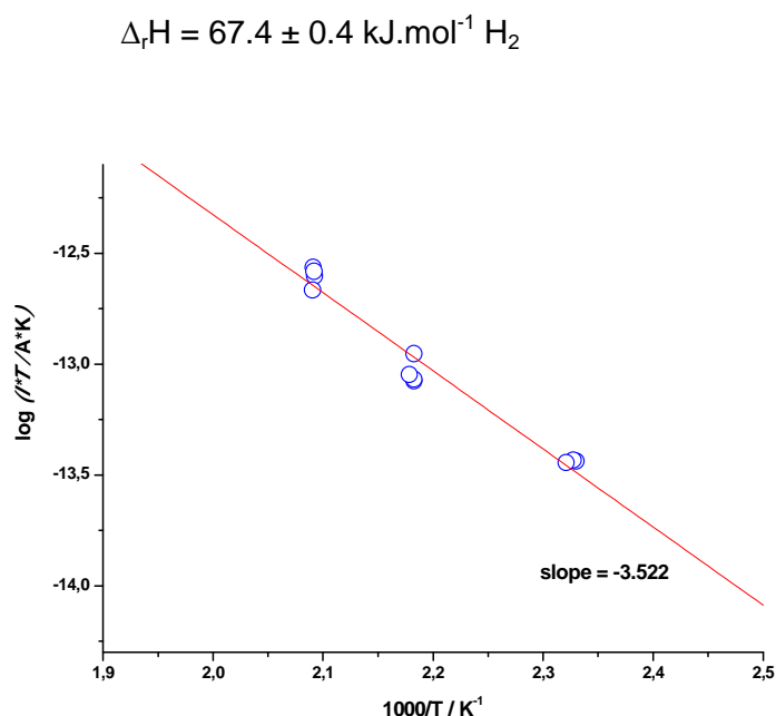
Figure 5.7. Logarithmic variation of the factor I^*T \propto \text{pressure} (for \text{H}_2 ) as a function of the inverse of the temperature.
