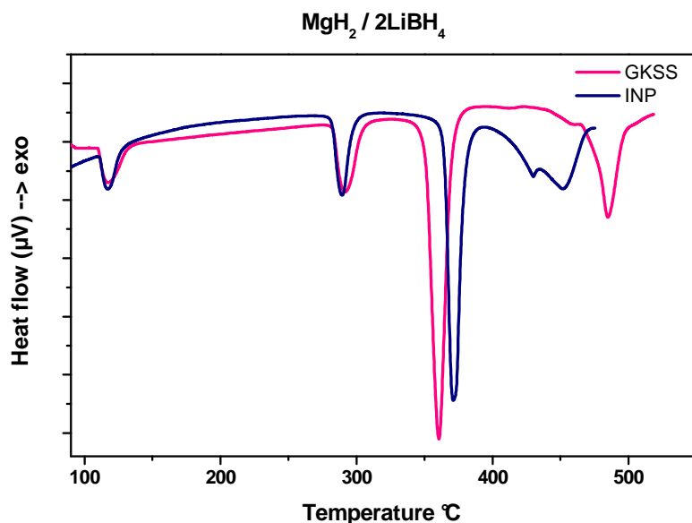
Figure 3.22. DSC analysis comparison of the hydride mixture at x = 2
