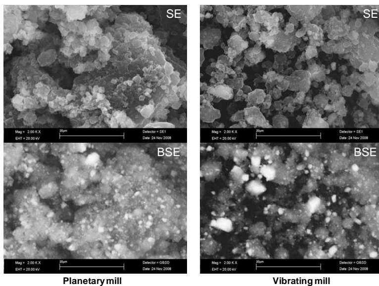
Figure 3.19. SEM Micrograph of MgH_2-2LiBH_4 prepared by planetary and vibrating mill in SE and BSE modes (Mag. \times 2 \cdot 10^3 )
