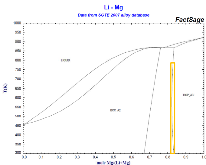
Figure 3.16. Li-Mg assessed phase diagram (computed with FactSage software)
