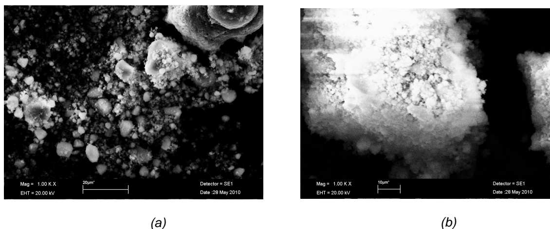
Figure 3.3. SEM micrograph of MgH_2 powder after several milling times (Magnification \times 1000 ): (a) 12 h, (b) 145 h
