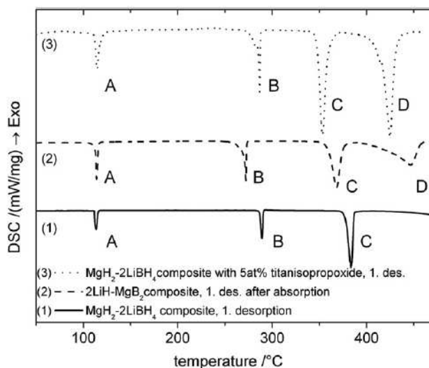
Figure 1.7. High Pressure-DSC of MgH_2+2LiBH_4 after (1) milling, (2) initial hydrogenation (3) Ti-isopropoxide addition (5 K.min^{-1} , 20 ml.min^{-1} and 3 bar H_2 ) [28]
