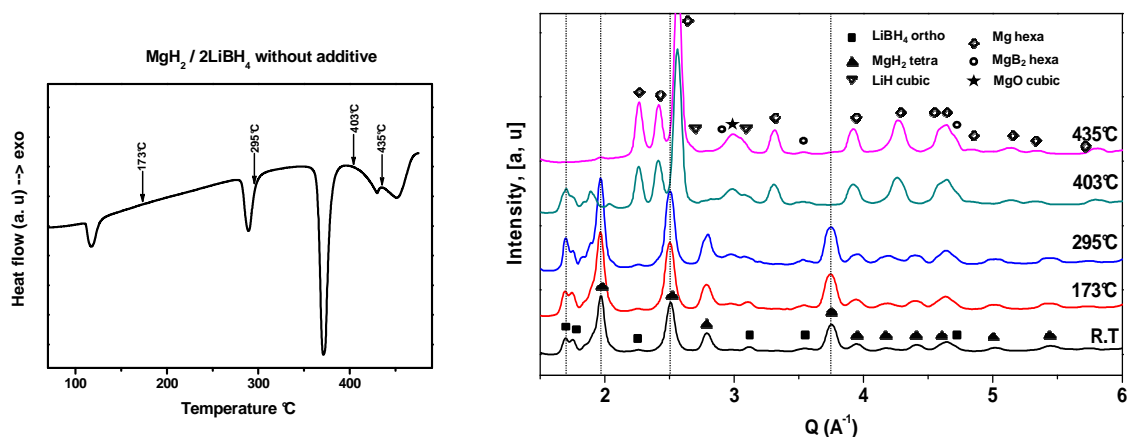
Figure 3.24. Room temperature X-ray reflections using synchrotron beam of the MgH 2 -2LiBH 4 hydride mixture upon temperature of annealing in DSC
