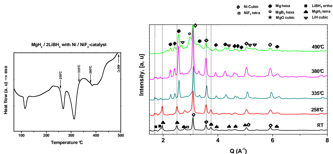
Figure 3.32. Room temperature X-ray reflections using synchrotron beam of the \text{MgH}_2\text{-2LiBH}_4 hydride mixture with Ni-based additive upon temperature of annealing in the DSC
