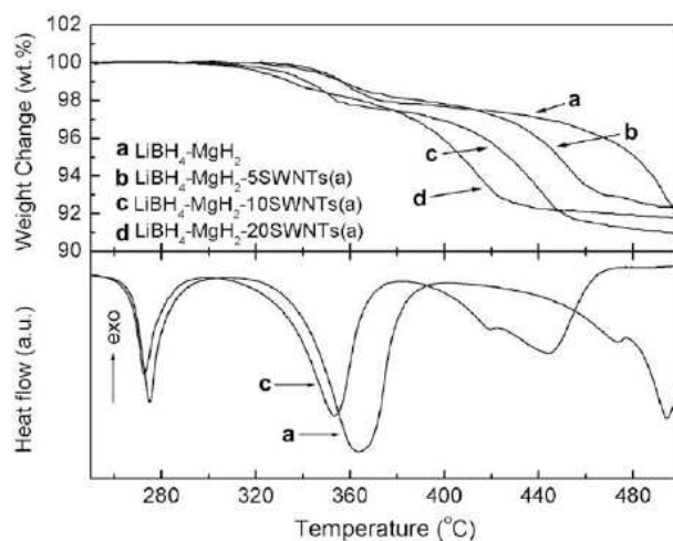
Figure 1.8. DSC of MgH_2+2LiBH_4 with addition of carbon nanotubes (SWNTs) under Ar gas flow at 10 K.min^{-1}
