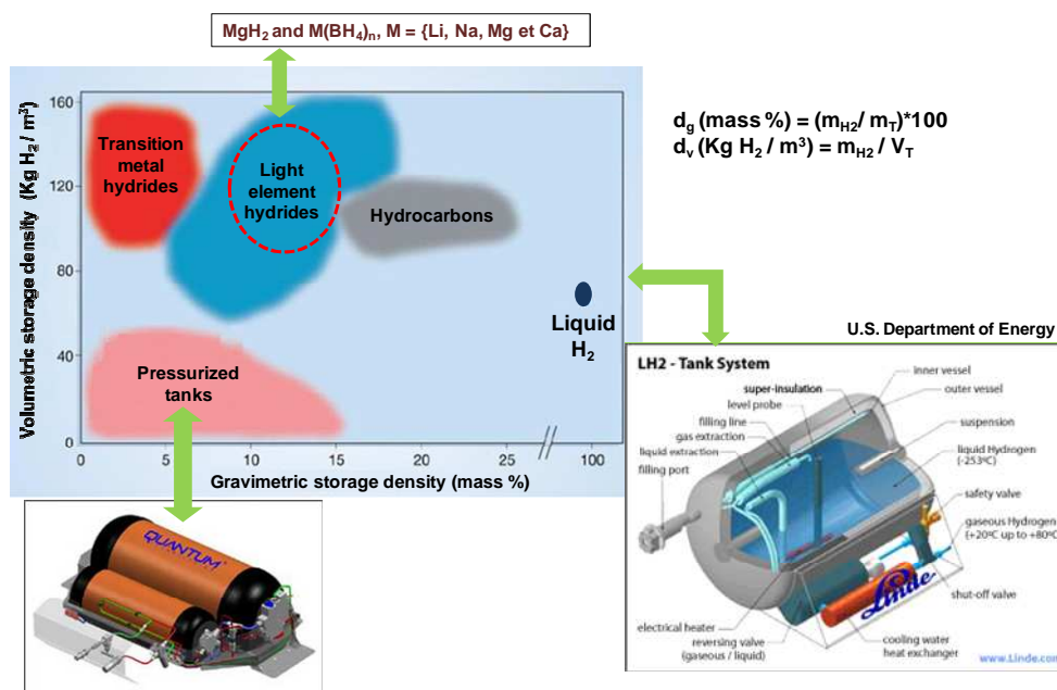
Figure 0.1. Hydrogen storage capacity. Volumetric (mass of H_2 per unit volume of storage medium) versus gravimetric (% H_2 storage density) values for different hydrogen storage systems 1,2
