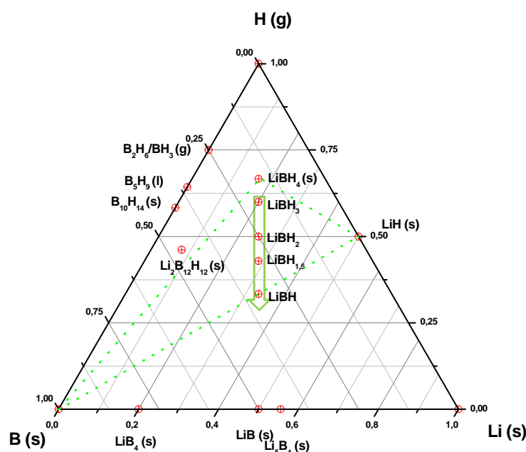
Figure 5.1. Schematics of the room temperature Li-B-H ternary phase diagram including \text{LiBH}_{4-x} hypothetical compounds
