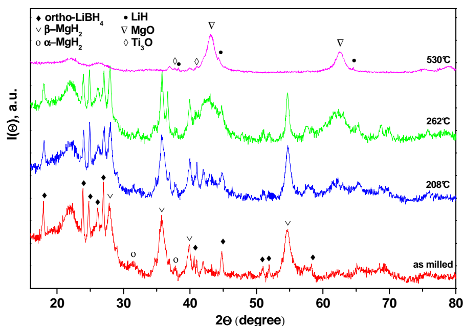
Figure 3.26. XRD patterns of MgH 2 -2LiBH 4 with Tiso as a function of the temperature
