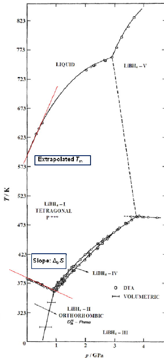
Figure 4.7. \text{LiBH}_4 high pressure p - T phase diagram deduced from Pistorius [23] data (the axes are transformed to the appropriate units): determination of the transition and melting temperatures by extrapolating at 0 GPa and extraction of the entropy of the phase transition from the slope of the boundary line.
