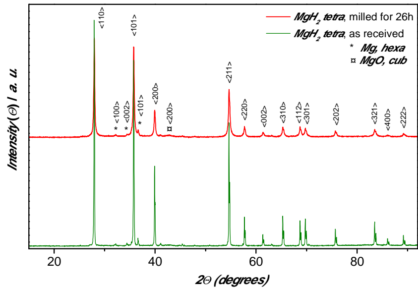
Figure 3.4. XRD pattern of MgH_2 as received and milled for 26 h
