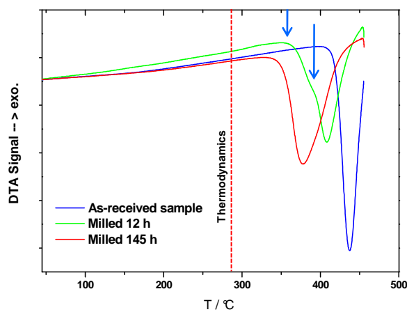
Figure 3.5. Thermal analysis (DTA) of MgH_2 milled at various milling times
