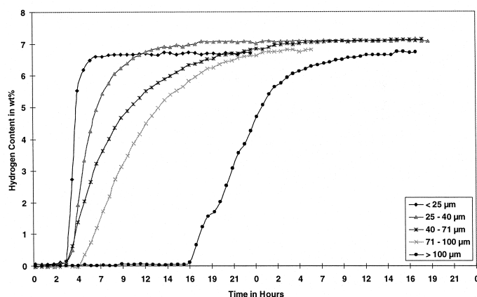
Figure 1.5. Progress of the hydrogenation of the Mg powder samples with different particle sizes at temperature 350°C and pressure up to 30 bar [40]
