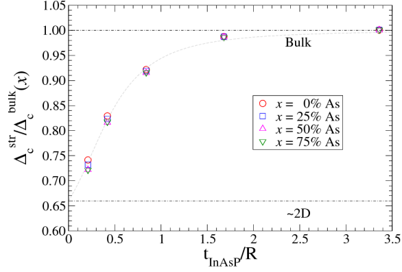
Figure 3.14: Normalized conduction band barrier InP/InAs - Normalized conduction band barrier height \Delta_c^{\text{str}}/\Delta_c^{\text{bulk}}(x) in InAs/InAs x P 1-x nanowire heterostructures as a function of t_{\text{InAsP}}/R , for various As concentrations x ( R = 10 nm). The bulk and 2D ( x = 1 ) barrier heights are reported on the figure. The dashed line is equation (3.53).
