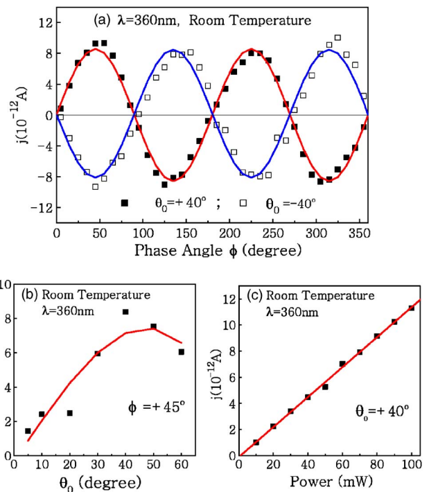
FIG. 2. (Color online) The current is measured through AA' contact pair for direction perpendicular to propagation of incident light ( \beta=90^\circ ). (a) The phase angle \phi dependence of CPGE photocurrent in the plane of GaN 2DEG sample (incident angle \theta_0=\pm 40^\circ ). (b) The incident angle \theta_0 dependence of the CPGE photocurrent with fixed radiation helicity. For both (a) and (b), the radiation power is 70 mW. (c) The dependence of the radiation power (incident angle \theta_0=40^\circ ). Measurements are carried out at room temperature and irradiation by light at the wavelength of 360 nm.
