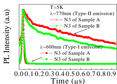
Figure 2. PL decays measured at 770nm (Type-II emission) and 600nm (Type-I emission) by TRPL. The curve in red is for the data of “linear” CdTe/CdSe/CdTe heterostructure nanorods samples-A N3; the curve in green is for the data of “core-shell” CdTe/CdSe/CdTe heterostructure nanorods samples-B N3. All the data were obtained at 5K.
