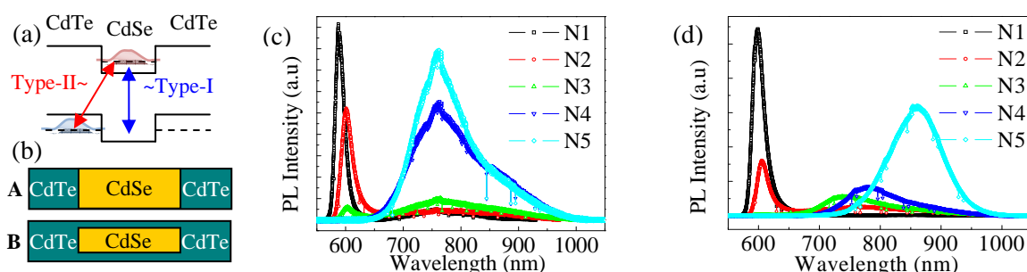
Figure 1. (a) Type-II band alignment at the interface between CdSe and CdTe; (b) The geometrical structure of samples-A and -B; (c) PL of CdSe seed (N1) and samples-A (from N2 to N5); (d) PL of CdSe seed (N1) and samples-B (from N2 to N5); All the data were obtained at 5K.
