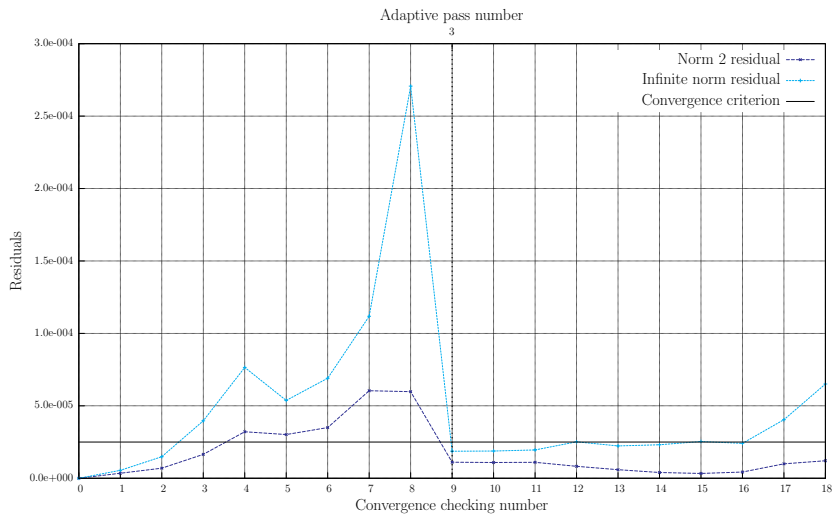
Figure 3.14 History of the check of the adaptive passes convergence all along the helicopter round robin analysis. The vertical dotted lines represent the creation of the successive passes during the computations.
