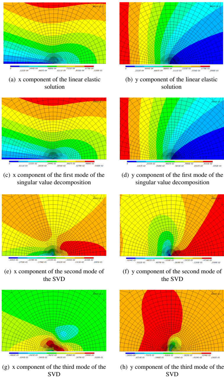
Figure 1.19 Displacement fields obtained by a linear elastic computation of a 2D crack in mode I (a) - (b), and 3 first modes of the singular value decomposition of the field history of the same crack with an elastic-plastic behavior (c) to (h). The linear elastic solution is very close to the first mode of the SVD.
