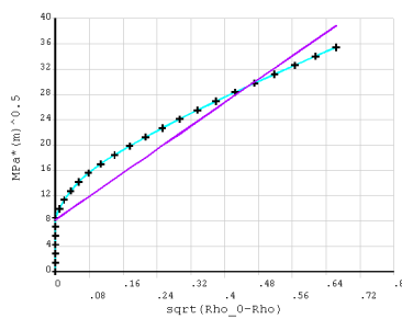
(a) Curve obtained by finite element computation (in green) and least square fit (in purple) represented in a (K_0^\infty - K^\infty) - (\sqrt{\rho_0 - \rho}) chart.
