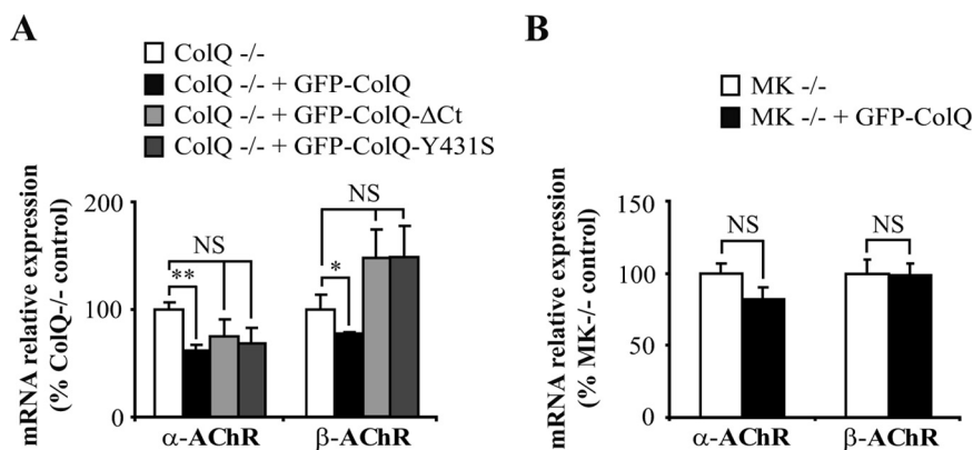
Figure 7. ColQ-dependent regulation of AChR mRNA levels is mediated by ColQ-MuSK interaction. A, B. Quantification of \alpha - and \beta -AChR mRNA levels by real-time RT-PCR. Levels of mRNAs are represented as relative expression ( 2^{-\Delta\Delta Ct} versus reference gene \times 100 ). A. \alpha - and \beta -AChR mRNA levels were decreased in ColQ -/- transfected with GFP-ColQ but not in cells transfected with GFP-ColQ- \Delta Ct or GFP-ColQ-Y431S. B. \alpha - and \beta -AChR mRNA levels were not modified by GFP-ColQ overexpression in MuSK-deficient myotubes (MK -/- ). Data are presented as percentage of control \pm SEM from three to five independent experiments. * p < 0.05 ; ** p < 0.01 ; NS, not significant; unpaired Mann-Whitney's U test.
