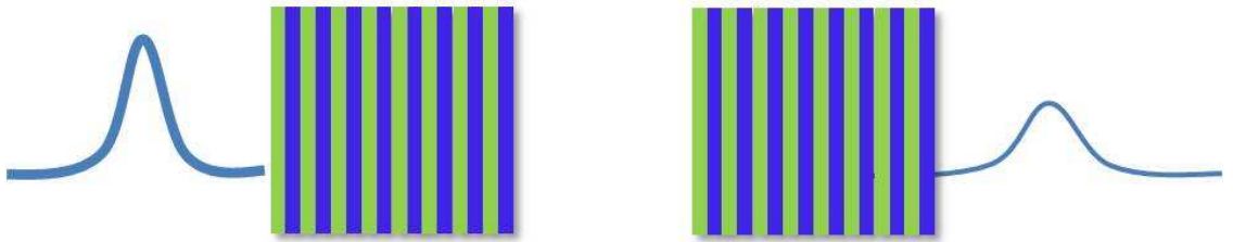
Fig. 2.1: Schematic of optical tunneling on 1D photonic structure
