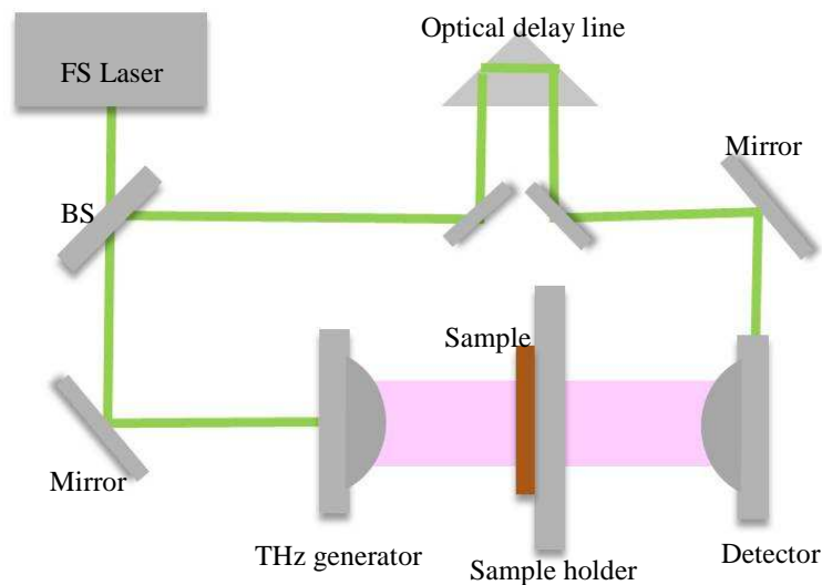
Fig. 5.16: The experiment setup of THz-TDS.
