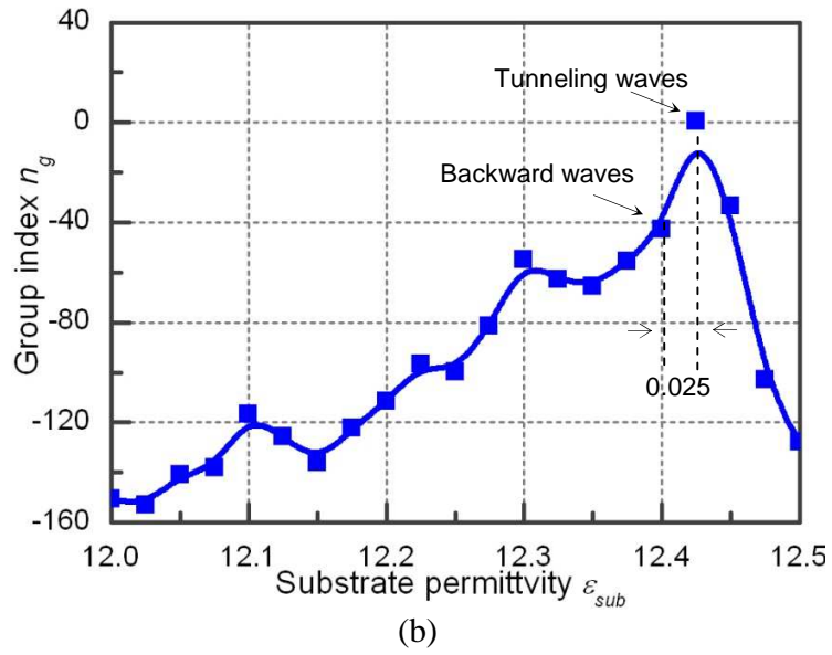
Fig. 4.17: The group index as a function of the substrate permittivity. The incidence frequency is 43.73 THz. The propagated light is tuned from a slowed backward wave to a
