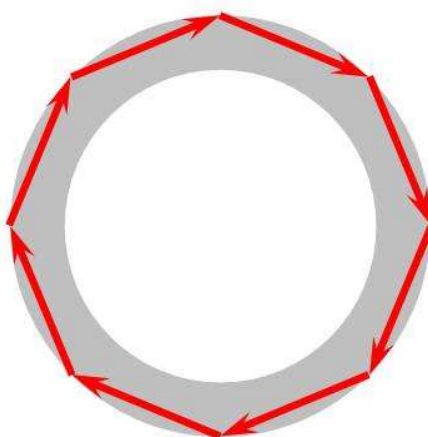
Fig. 2.4: Schematic of whispering gallery mode (WGM) micro-cavity.
