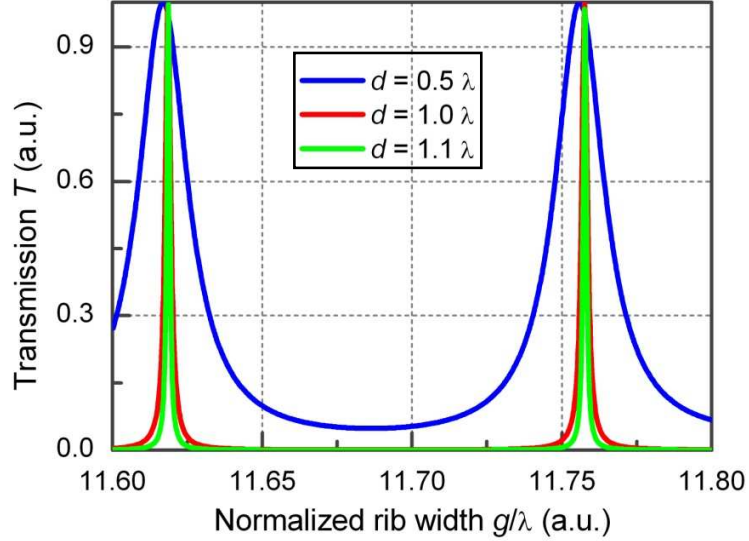
Fig. 3.11: The transmission versus the central rib width g .
