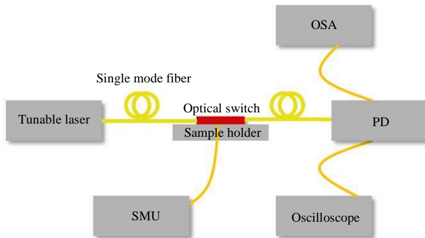
Fig. 3.16: Experimental setup of the thermo-optical switch
