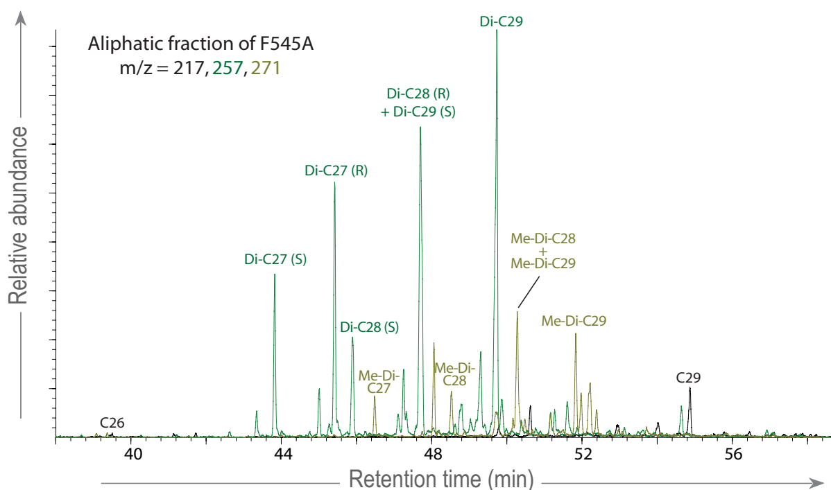
Fig. 5.11. Chromatogram of the aliphatic fraction of the sample F545a ( m/z 217, 257, 271). Diasterenes and methylsteranes peaks are predominant. C26 to C29 : regular steranes having from 26 to 29 carbon atoms; Di-C27 to Di-C29 : diasterenes having from 27 to 29 carbon atoms; Me-Di-C27 to Me-Di-C29 : methylsteranes having from 27 to 29 carbon atoms.
