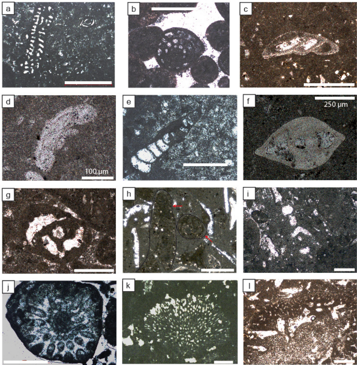
Fig. 6 Microfossils of the Upper Oxfordian-Lower Kimmeridgian from the Gudmont-Villiers section. a Labyrinthina mirabilis Weinschenk and Labalina (Calcaires crayeux de Gudmont Formation). b Nautiloculina oolithica Mohler (CCG Formation). c Mohlerina basiliensis (Mohler)(Calcaires À serpules de Gudmont Formation). d Hungarillina pedunculata Blau & Wernli (Calcaires À serpules de Gudmont Formation). e Troglotella incrustans Wernli & Fuchs in Cladocoropsis mirabilis Felix (Calcaires crayeux de Gudmont Formation). f Pink Lenticulina (Calcaires à astartes Formation). g , i Everticyclammina virguliana (Koechlin) (CCG Formation & Oolithe de Lamothe Formation). h Alveosepta jaccardi (Schrodt) (CCG Formation). j Dasycladacean ( Salpingoporella annulata Carozzi?) G6. k Cayeuxia pia Frolo (G'9). l Lithocodium aggregatum Elliott (Calcaires crayeux de Gudmont Formation). When the scale is not precised, the segment measures 500 µm.
