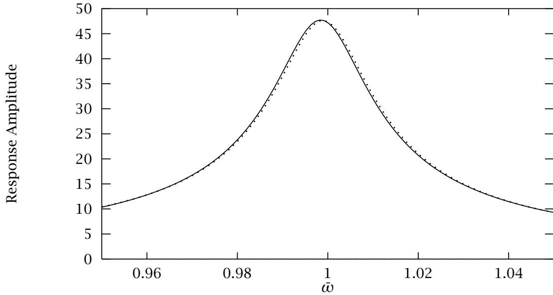
Figure 7.16 Frequency response of tuned assemblies of types 1Bc (—) and 1Bd (·····) for engine order 22 excitation.
