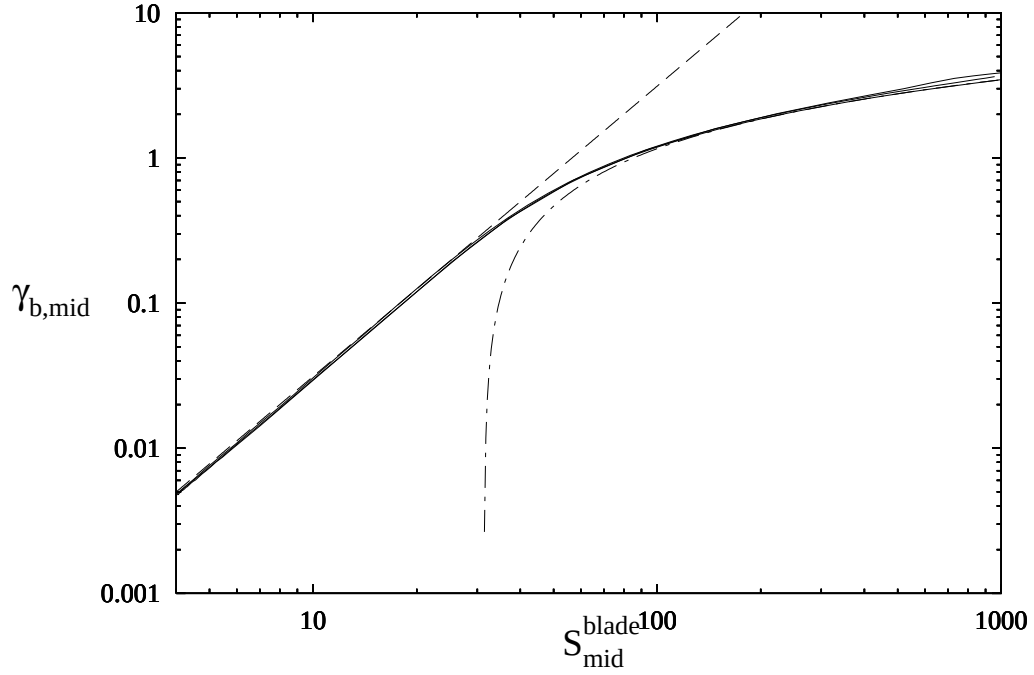
Figure 5.10 Monte Carlo simulations ( — ) are used to verify Eq. (5.63) ( - - - ) and Eq. (5.65) ( — · — ). Multiple Monte Carlo simulations are obtained by varying \bar{m} in 1 st passband, \bar{k}_d in 2 nd passband and \bar{k}_c in 1 st passband. The standard deviation of blade stiffness mistuning is 5%. Note the near overlap of the various Monte Carlo results.
