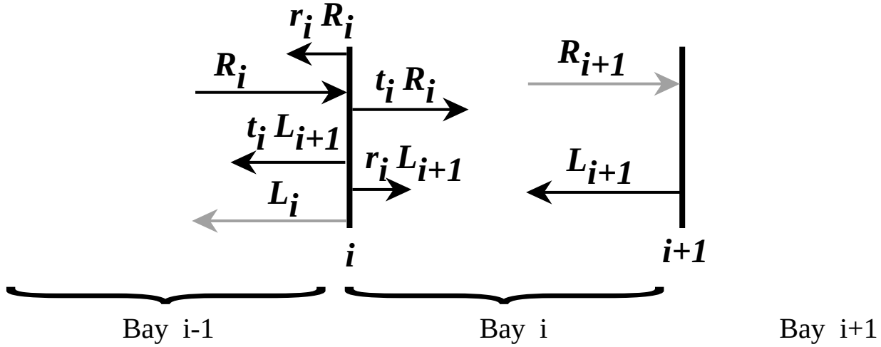
Figure 5.5 Scattering of waves at substructure interfaces in a structure with a single wave channel.
