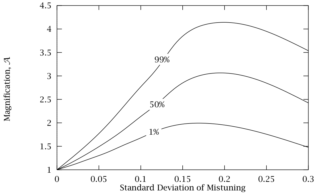
Figure 7.31 Magnification of largest amplitude due to mistuning as a function of the standard deviation of blade stiffness mistuning, s , for model 3Ba. The curves show the 1%, 50% and 99% percentiles of the statistics of forced response obtained by a frequency sweep. Engine order of the excitation is 7.
