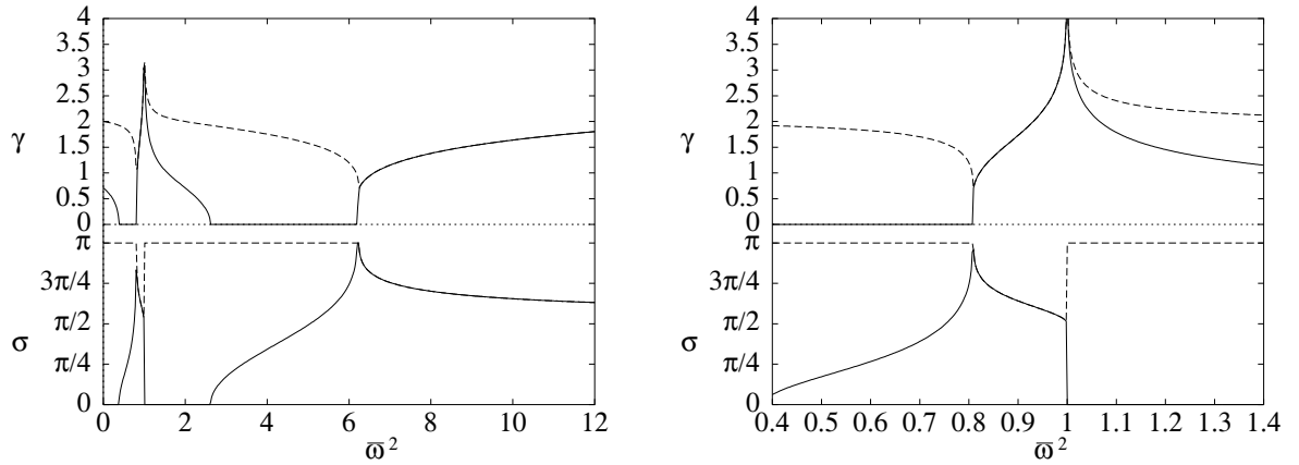
Figure 5.3 Propagation constants vs. frequency for the system in Fig. 3.13 with \bar{m} = 1 , \bar{k}_d = 1 , \bar{k}_{c1} = 1 and \bar{k}_{c2} = 0.2 . A detailed view on the right. Wave type one is (—) and type two is (---).
