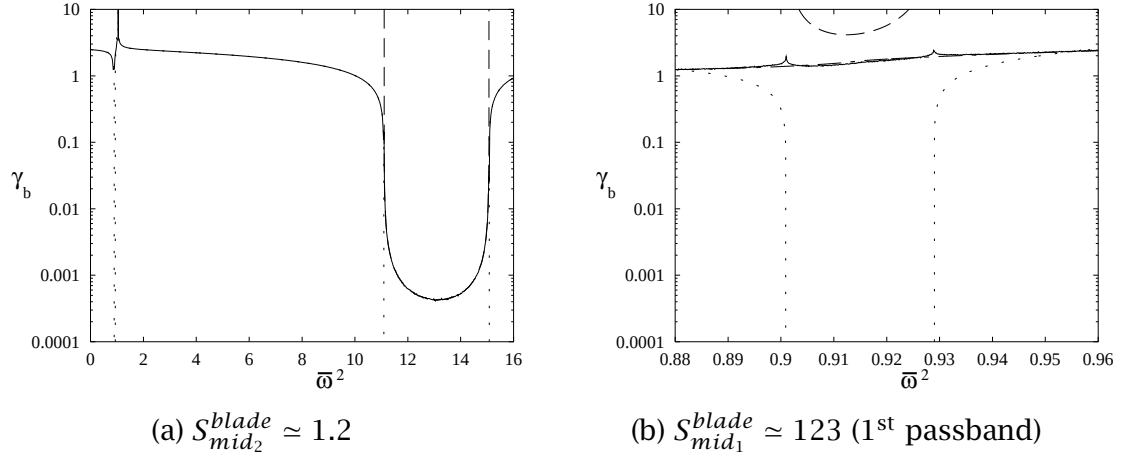
Figure 5.11 Exponential decay, \gamma_b , due to 5% blade stiffness mistuning vs. frequency. In stopbands Monte Carlo simulations (—) agree with the propagation constant for the tuned system (·····). In (a) the simulations results overlap the classical perturbation result (---), Eq. (5.62), in the 2 nd passband. In (b) the simulation agrees with the modified perturbation result (- - -), Eq. (5.64).
