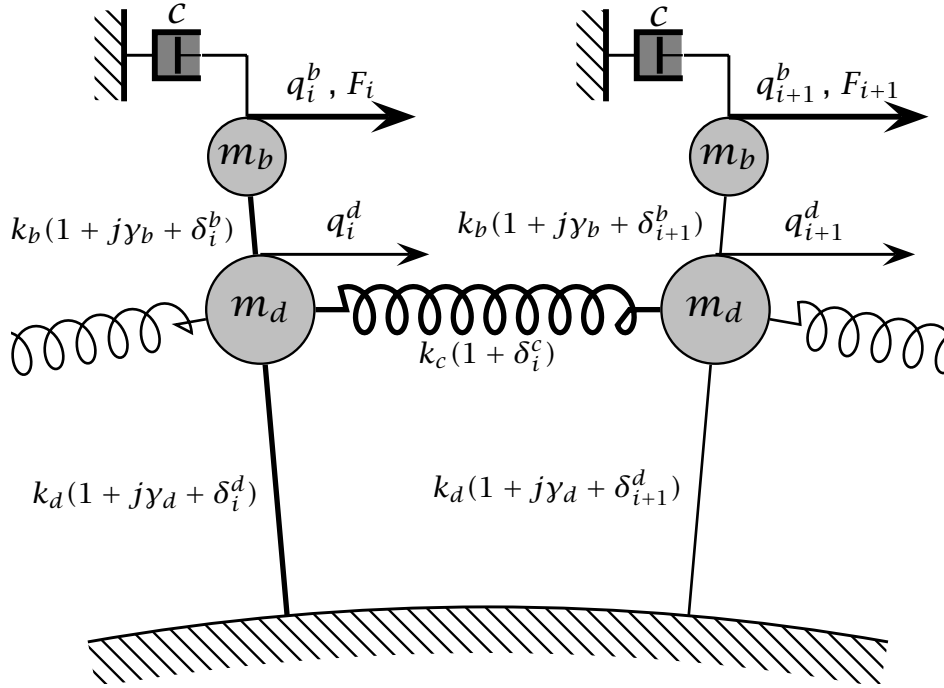
Figure 3.4 A simple model of a bladed disk featuring one disk-DOF and one blade-DOF, mono-coupled bays to model each blade/disk sector.
